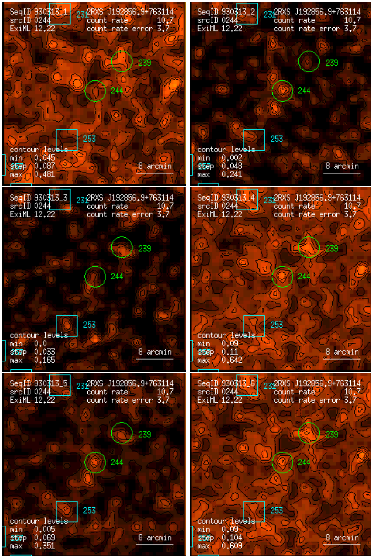
Figure 244: RASS 930313: detection 0244: band rate images, Gaussian filter: (1) PSPC channels 11 – 41, (2) 52 – 90, (3) 91 – 201, (4) 11 – 235, (5) 52 – 201, (6) 11 – 201. Broad band rates in counts/ks. Band rate contour levels in counts/ks/arcmin 2 .
