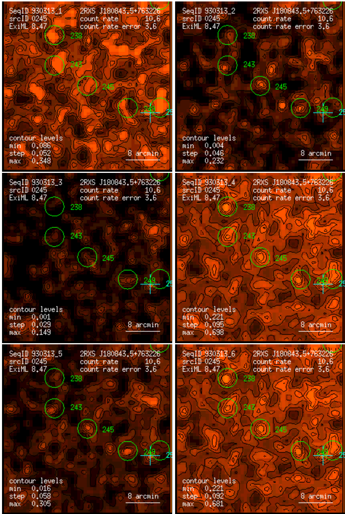
Figure 245: RASS 930313: detection 0245: band rate images, Gaussian filter: (1) PSPC channels 11 – 41, (2) 52 – 90, (3) 91 – 201, (4) 11 – 235, (5) 52 – 201, (6) 11 – 201. Broad band rates in counts/ks. Band rate contour levels in counts/ks/arcmin 2 .
