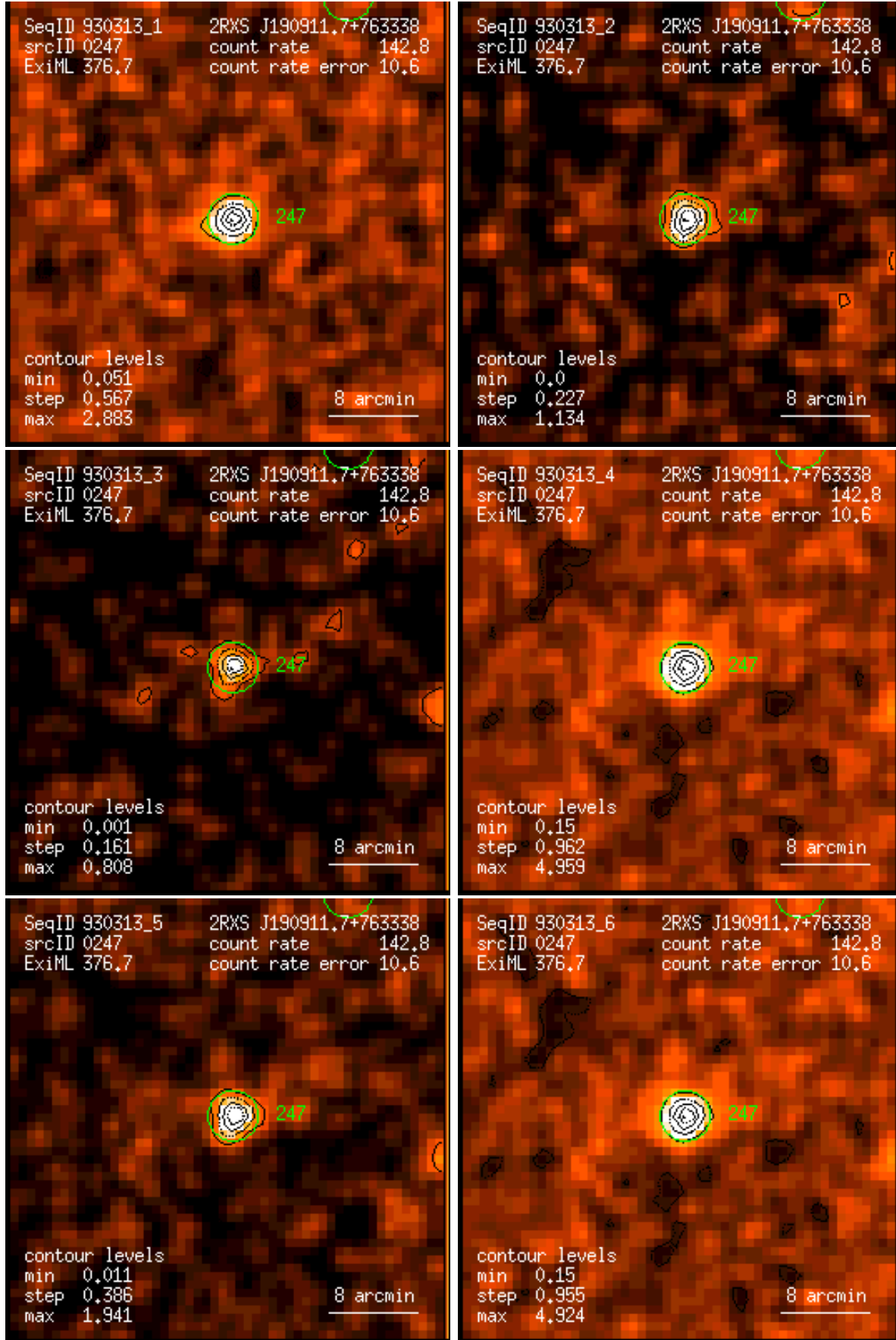
Figure 247: RASS 930313: detection 0247: band rate images, Gaussian filter: (1) PSPC channels 11 – 41, (2) 52 – 90, (3) 91 – 201, (4) 11 – 235, (5) 52 – 201, (6) 11 – 201. Broad band rates in counts/ks. Band rate contour levels in counts/ks/arcmin 2 .
