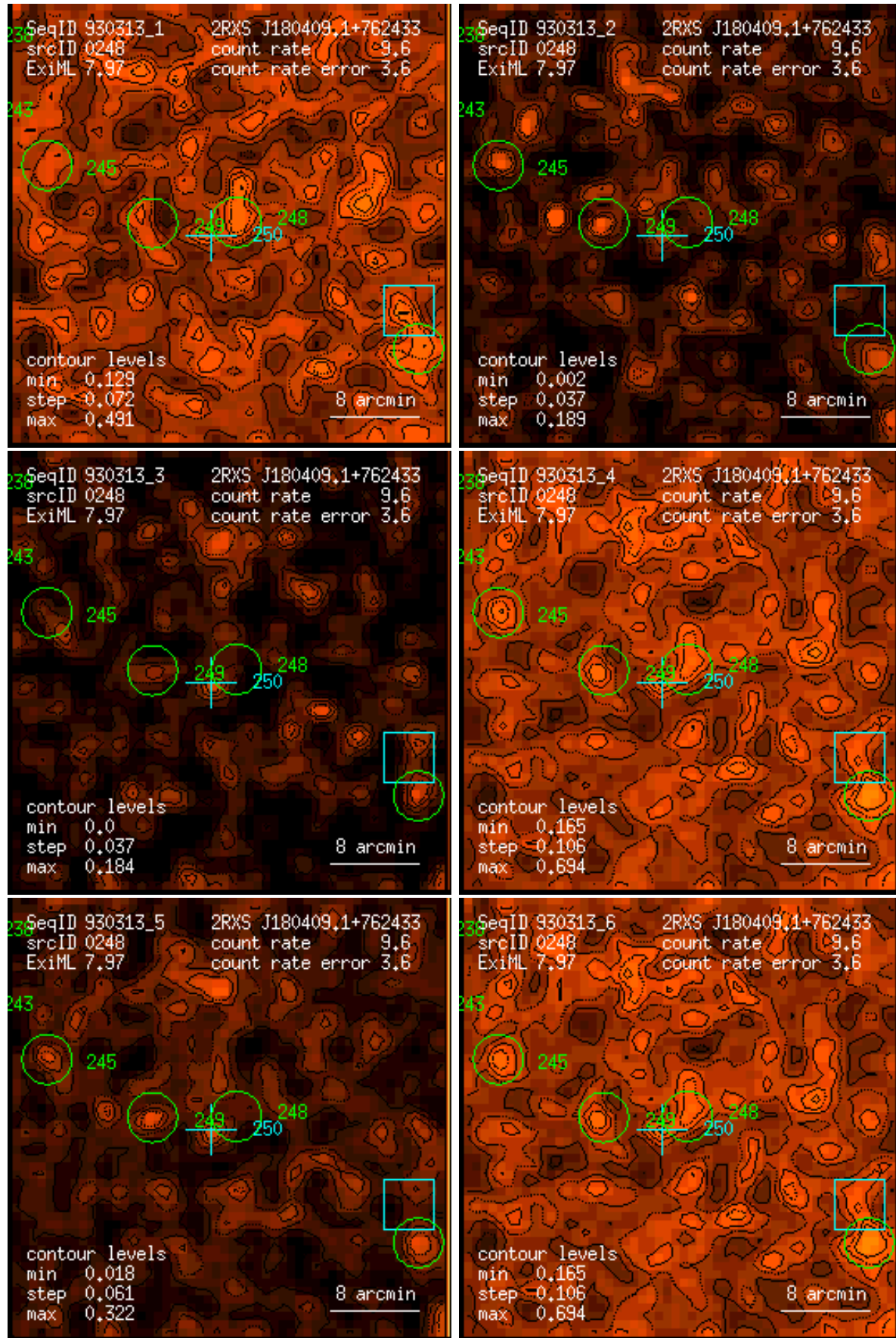
Figure 248: RASS 930313: detection 0248: band rate images, Gaussian filter: (1) PSPC channels 11 – 41, (2) 52 – 90, (3) 91 – 201, (4) 11 – 235, (5) 52 – 201, (6) 11 – 201. Broad band rates in counts/ks. Band rate contour levels in counts/ks/arcmin 2 .
