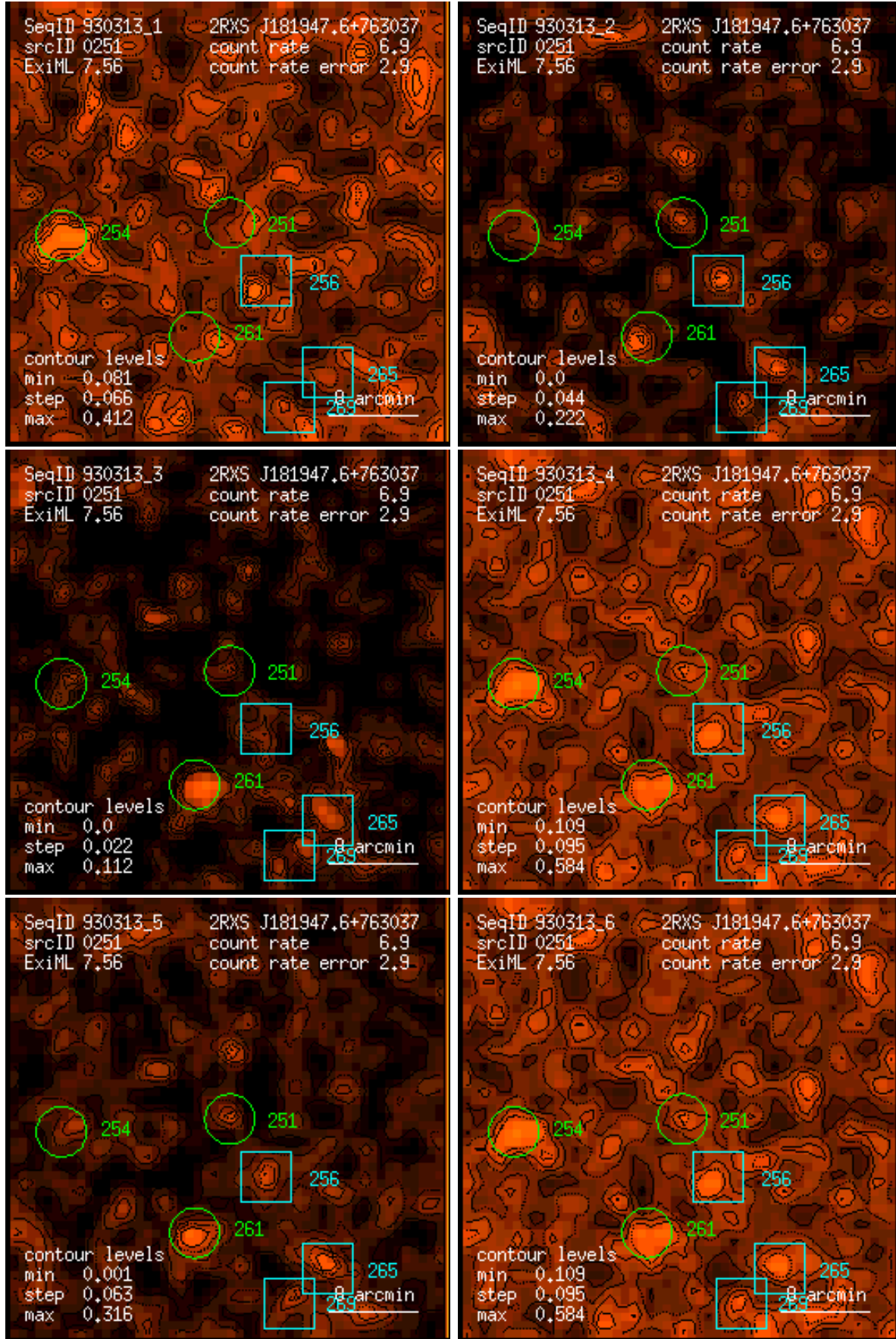
Figure 251: RASS 930313: detection 0251: band rate images, Gaussian filter: (1) PSPC channels 11 – 41, (2) 52 – 90, (3) 91 – 201, (4) 11 – 235, (5) 52 – 201, (6) 11 – 201. Broad band rates in counts/ks. Band rate contour levels in counts/ks/arcmin 2 .
