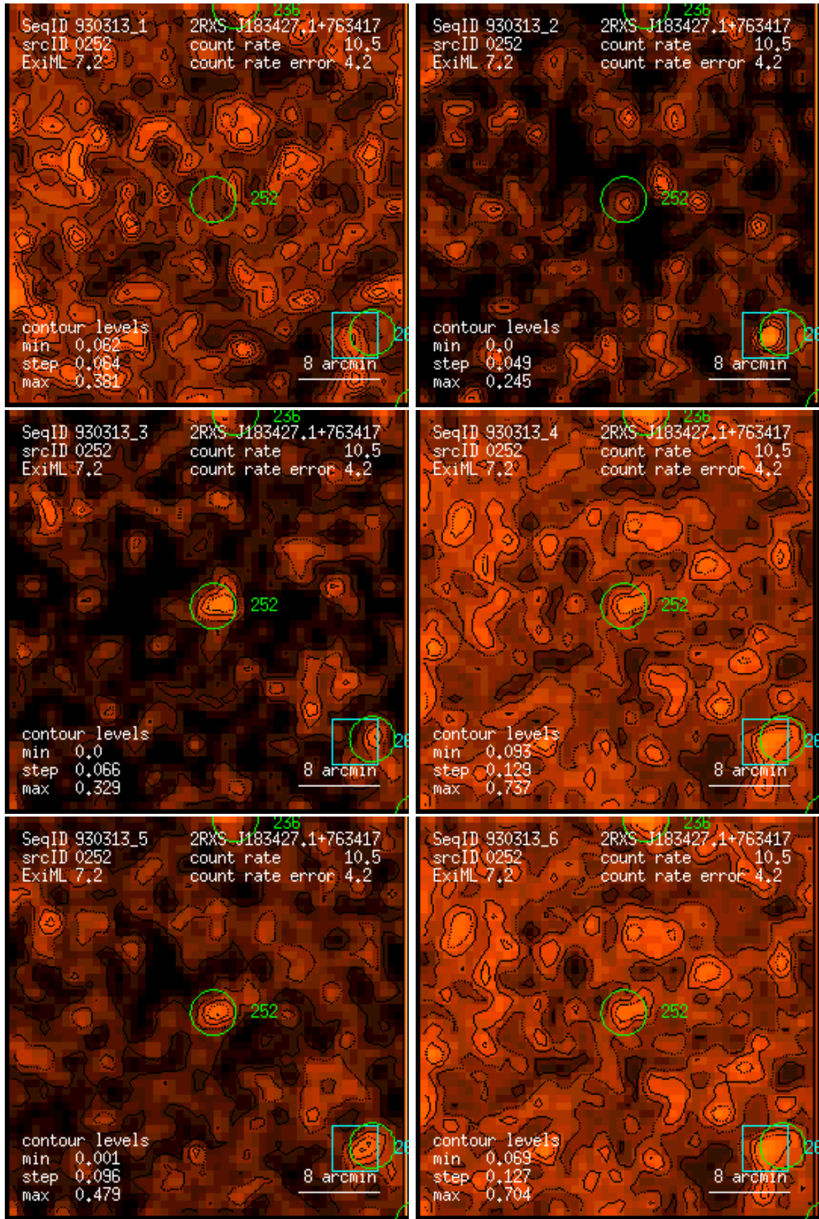
Figure 252: RASS 930313: detection 0252: band rate images, Gaussian filter: (1) PSPC channels 11 – 41, (2) 52 – 90, (3) 91 – 201, (4) 11 – 235, (5) 52 – 201, (6) 11 – 201. Broad band rates in counts/ks. Band rate contour levels in counts/ks/arcmin 2 .
