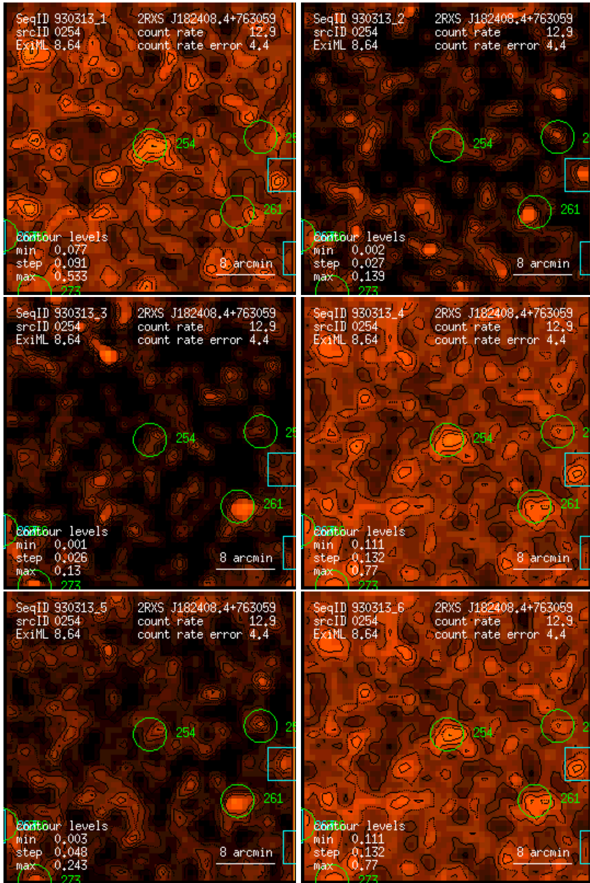
Figure 254: RASS 930313: detection 0254: band rate images, Gaussian filter: (1) PSPC channels 11 – 41, (2) 52 – 90, (3) 91 – 201, (4) 11 – 235, (5) 52 – 201, (6) 11 – 201. Broad band rates in counts/ks. Band rate contour levels in counts/ks/arcmin 2 .
