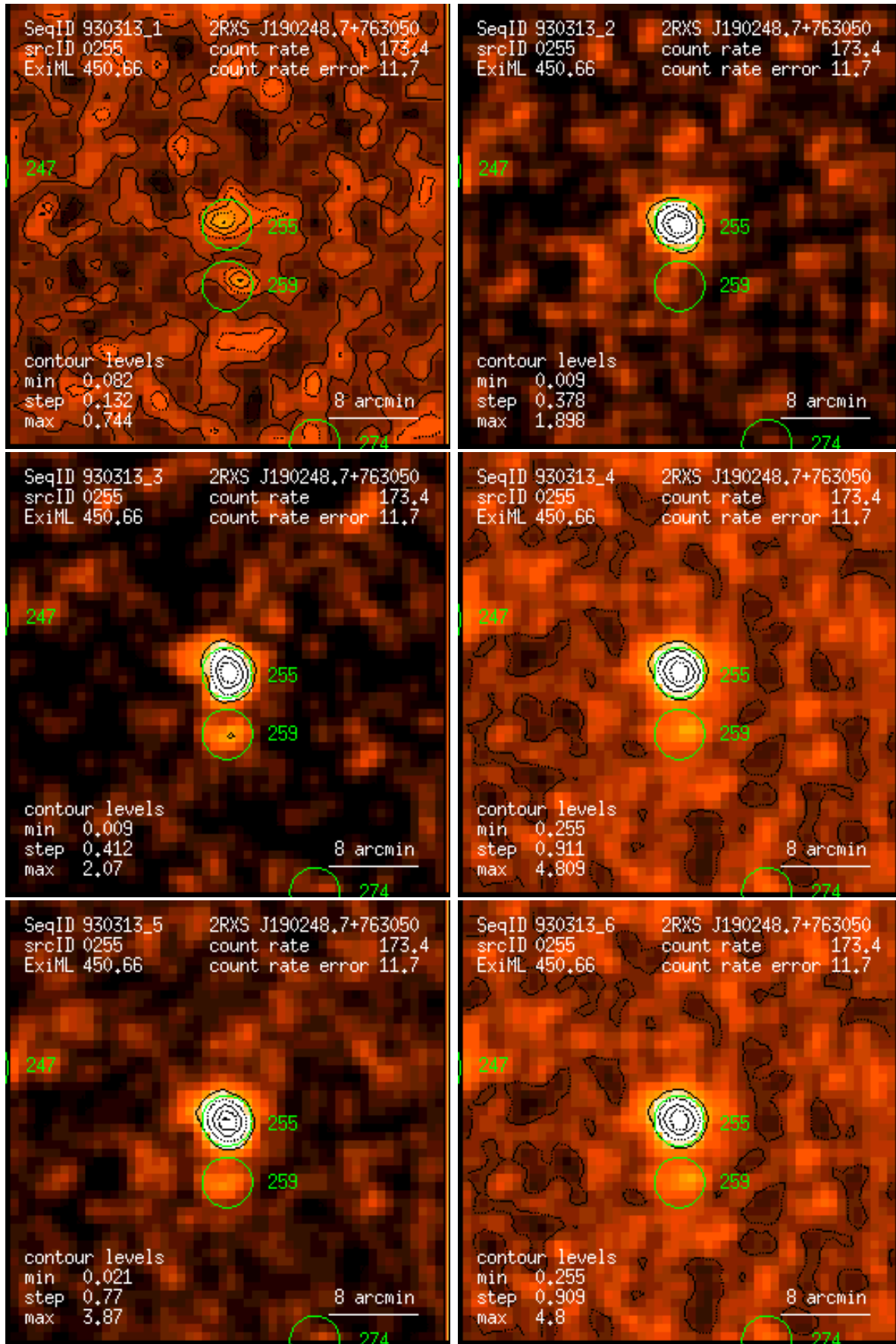
Figure 255: RASS 930313: detection 0255: band rate images, Gaussian filter: (1) PSPC channels 11 – 41, (2) 52 – 90, (3) 91 – 201, (4) 11 – 235, (5) 52 – 201, (6) 11 – 201. Broad band rates in counts/ks. Band rate contour levels in counts/ks/arcmin 2 .
