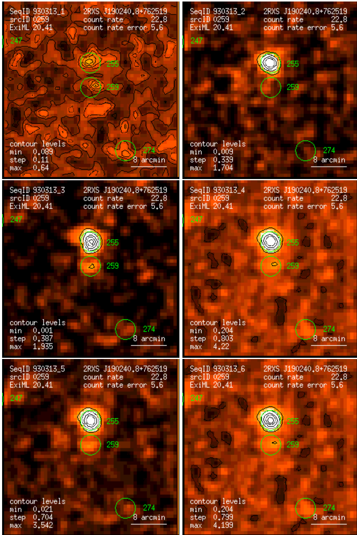
Figure 259: RASS 930313: detection 0259: band rate images, Gaussian filter: (1) PSPC channels 11 – 41, (2) 52 – 90, (3) 91 – 201, (4) 11 – 235, (5) 52 – 201, (6) 11 – 201. Broad band rates in counts/ks. Band rate contour levels in counts/ks/arcmin 2 .
