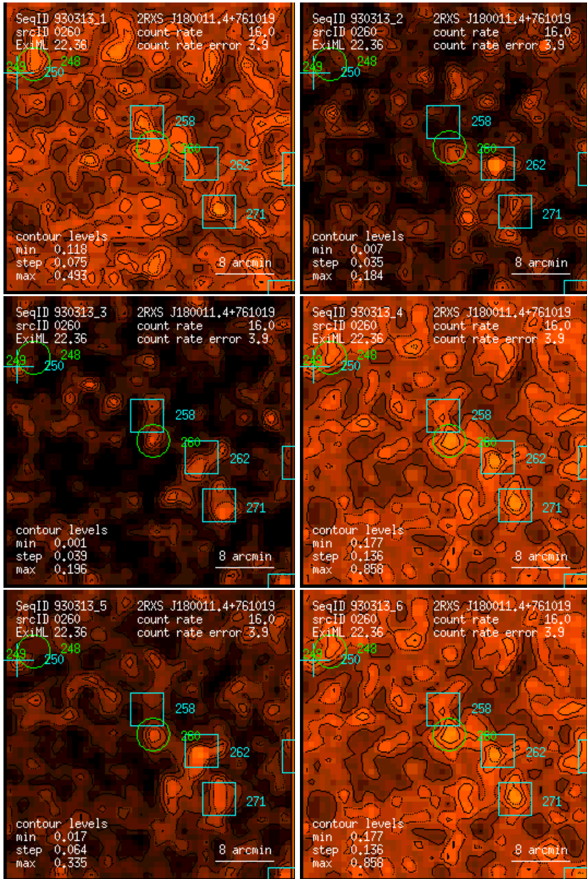
Figure 260: RASS 930313: detection 0260: band rate images, Gaussian filter: (1) PSPC channels 11 – 41, (2) 52 – 90, (3) 91 – 201, (4) 11 – 235, (5) 52 – 201, (6) 11 – 201. Broad band rates in counts/ks. Band rate contour levels in counts/ks/arcmin 2 .
