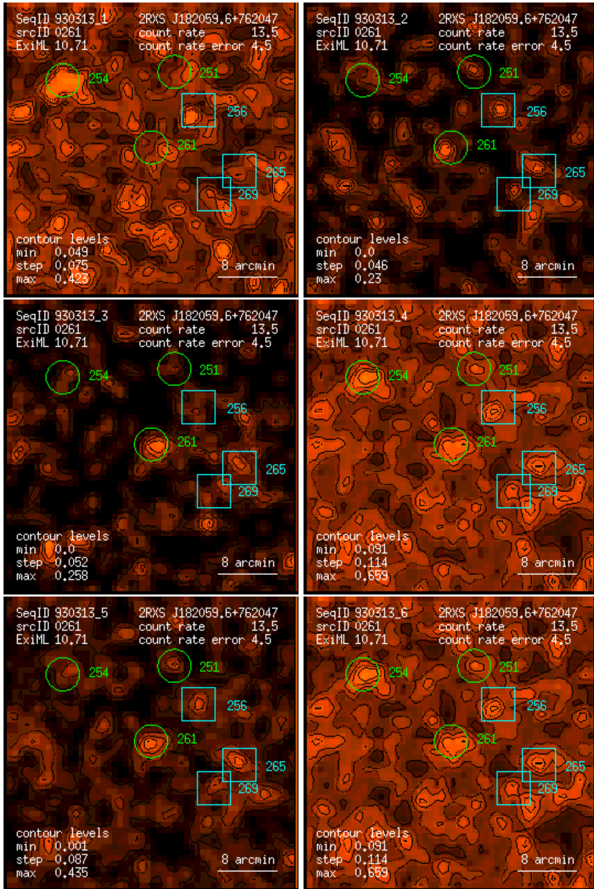
Figure 261: RASS 930313: detection 0261: band rate images, Gaussian filter: (1) PSPC channels 11 – 41, (2) 52 – 90, (3) 91 – 201, (4) 11 – 235, (5) 52 – 201, (6) 11 – 201. Broad band rates in counts/ks. Band rate contour levels in counts/ks/arcmin 2 .
