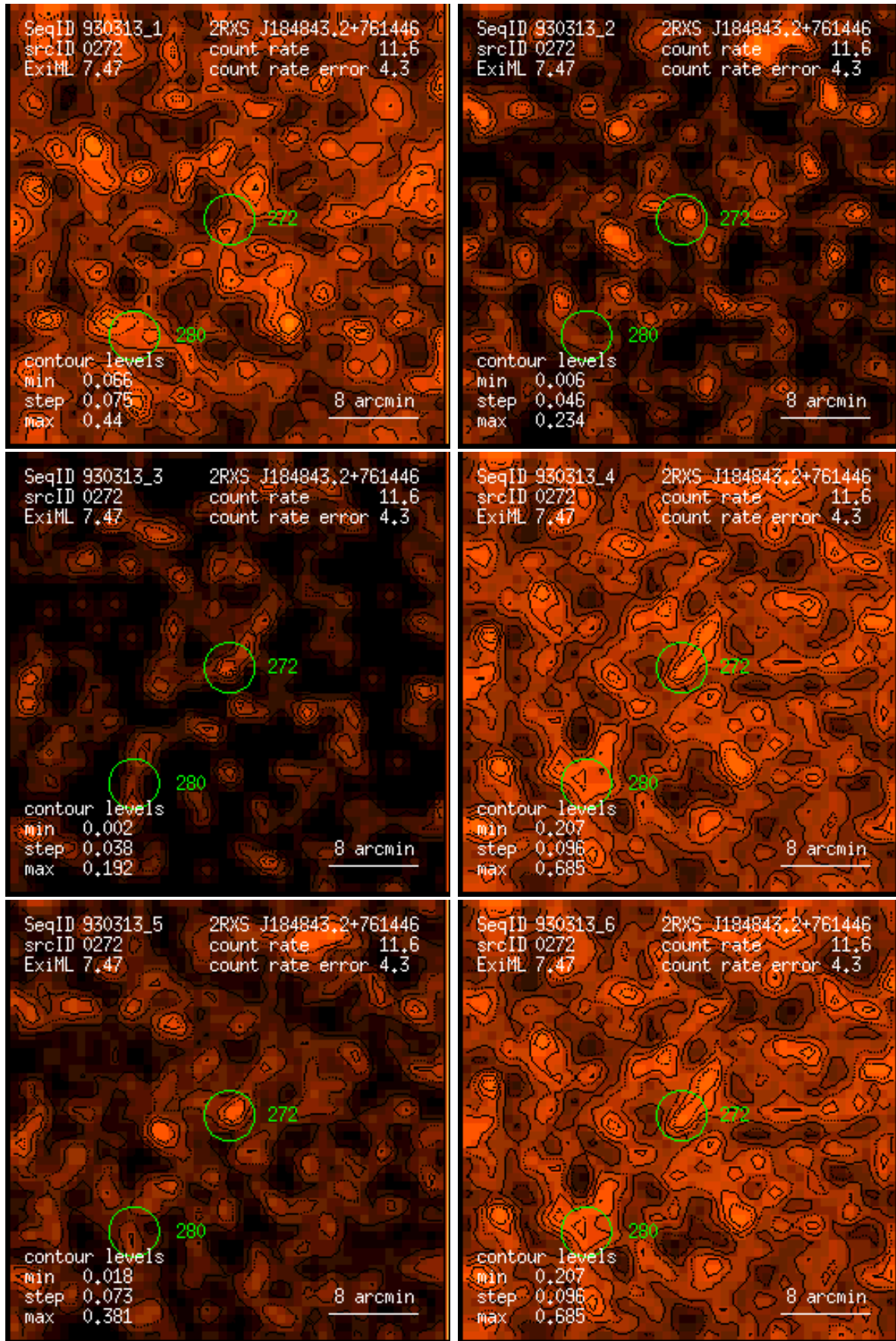
Figure 272: RASS 930313: detection 0272: band rate images, Gaussian filter: (1) PSPC channels 11 – 41, (2) 52 – 90, (3) 91 – 201, (4) 11 – 235, (5) 52 – 201, (6) 11 – 201. Broad band rates in counts/ks. Band rate contour levels in counts/ks/arcmin 2 .
