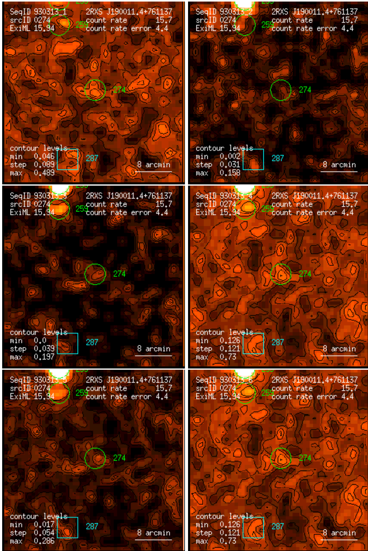
Figure 274: RASS 930313: detection 0274: band rate images, Gaussian filter: (1) PSPC channels 11 – 41, (2) 52 – 90, (3) 91 – 201, (4) 11 – 235, (5) 52 – 201, (6) 11 – 201. Broad band rates in counts/ks. Band rate contour levels in counts/ks/arcmin 2 .
