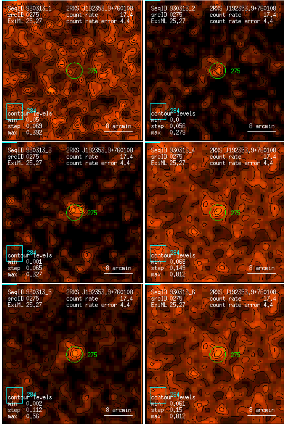
Figure 275: RASS 930313: detection 0275: band rate images, Gaussian filter: (1) PSPC channels 11 – 41, (2) 52 – 90, (3) 91 – 201, (4) 11 – 235, (5) 52 – 201, (6) 11 – 201. Broad band rates in counts/ks. Band rate contour levels in counts/ks/arcmin 2 .
