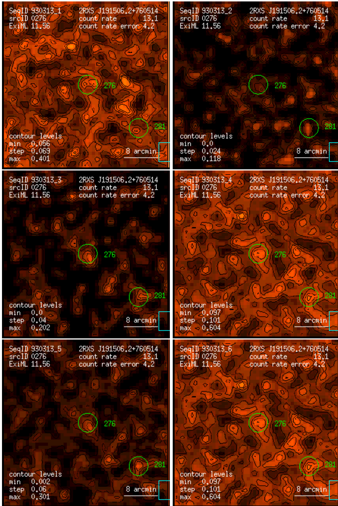
Figure 276: RASS 930313: detection 0276: band rate images, Gaussian filter: (1) PSPC channels 11 – 41, (2) 52 – 90, (3) 91 – 201, (4) 11 – 235, (5) 52 – 201, (6) 11 – 201. Broad band rates in counts/ks. Band rate contour levels in counts/ks/arcmin 2 .
