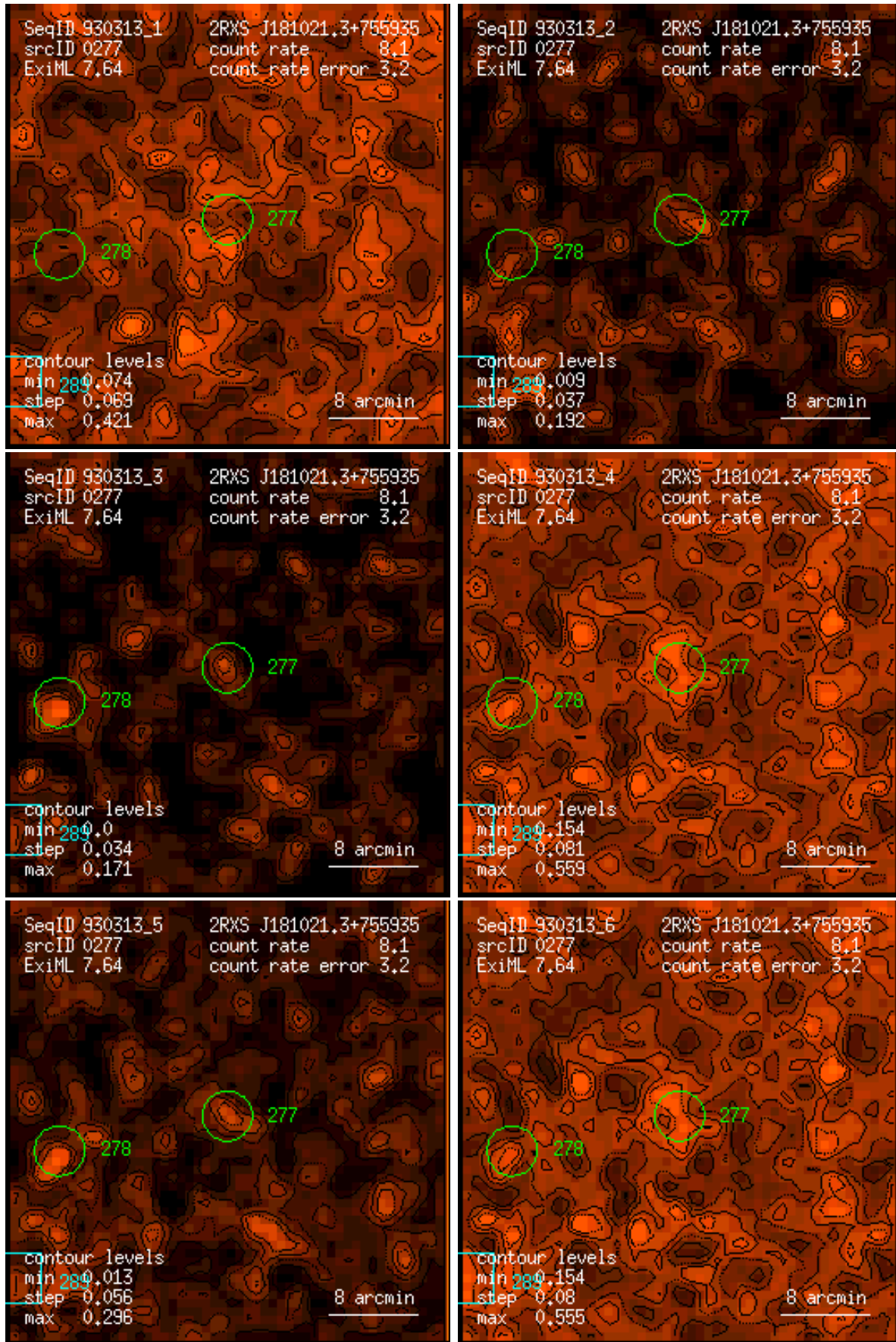
Figure 277: RASS 930313: detection 0277: band rate images, Gaussian filter: (1) PSPC channels 11 – 41, (2) 52 – 90, (3) 91 – 201, (4) 11 – 235, (5) 52 – 201, (6) 11 – 201. Broad band rates in counts/ks. Band rate contour levels in counts/ks/arcmin 2 .
