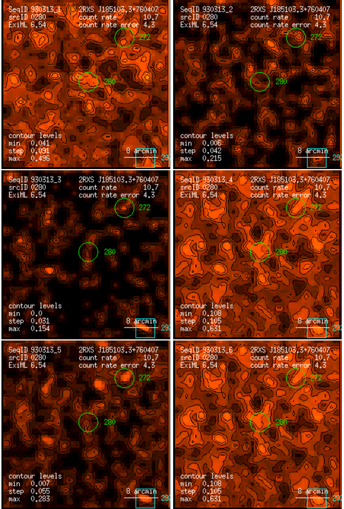
Figure 280: RASS 930313: detection 0280: band rate images, Gaussian filter: (1) PSPC channels 11 – 41, (2) 52 – 90, (3) 91 – 201, (4) 11 – 235, (5) 52 – 201, (6) 11 – 201. Broad band rates in counts/ks. Band rate contour levels in counts/ks/arcmin 2 .
