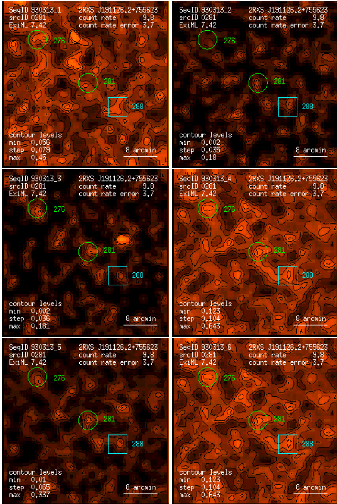
Figure 281: RASS 930313: detection 0281: band rate images, Gaussian filter: (1) PSPC channels 11 – 41, (2) 52 – 90, (3) 91 – 201, (4) 11 – 235, (5) 52 – 201, (6) 11 – 201. Broad band rates in counts/ks. Band rate contour levels in counts/ks/arcmin 2 .
