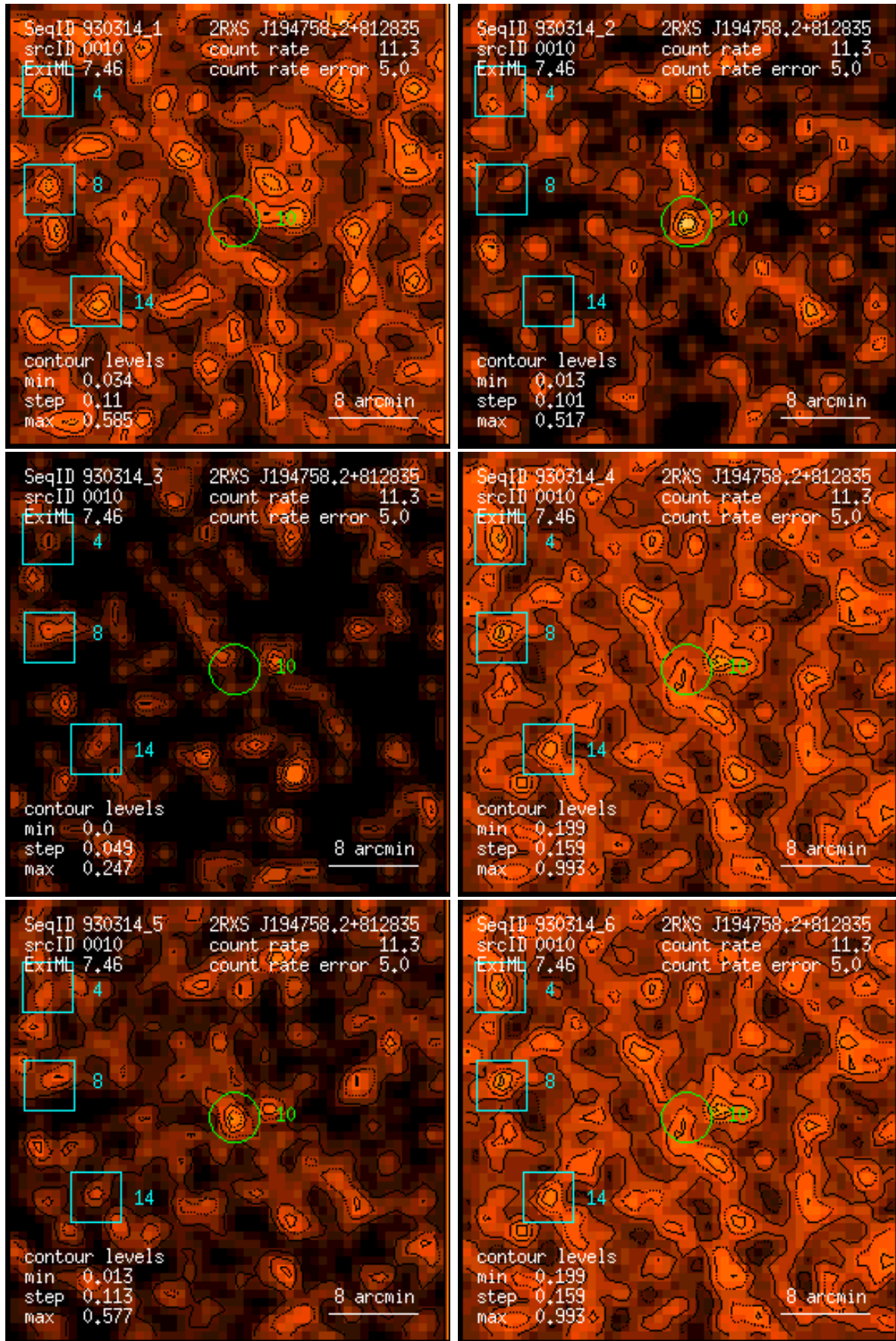
Figure 10: RASS 930314: detection 0010: band rate images, Gaussian filter: (1) PSPC channels 11 – 41, (2) 52 – 90, (3) 91 – 201, (4) 11 – 235, (5) 52 – 201, (6) 11 – 201. Broad band rates in counts/ks. Band rate contour levels in counts/ks/arcmin 2 .
