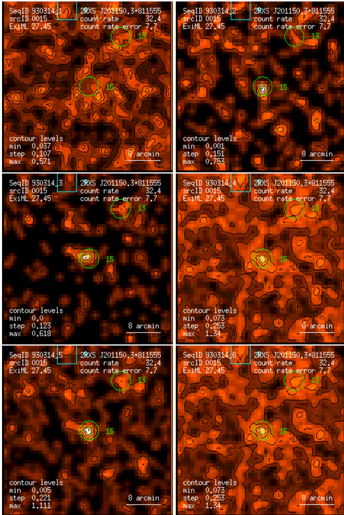
Figure 15: RASS 930314: detection 0015: band rate images, Gaussian filter: (1) PSPC channels 11 – 41, (2) 52 – 90, (3) 91 – 201, (4) 11 – 235, (5) 52 – 201, (6) 11 – 201. Broad band rates in counts/ks. Band rate contour levels in counts/ks/arcmin 2 .
