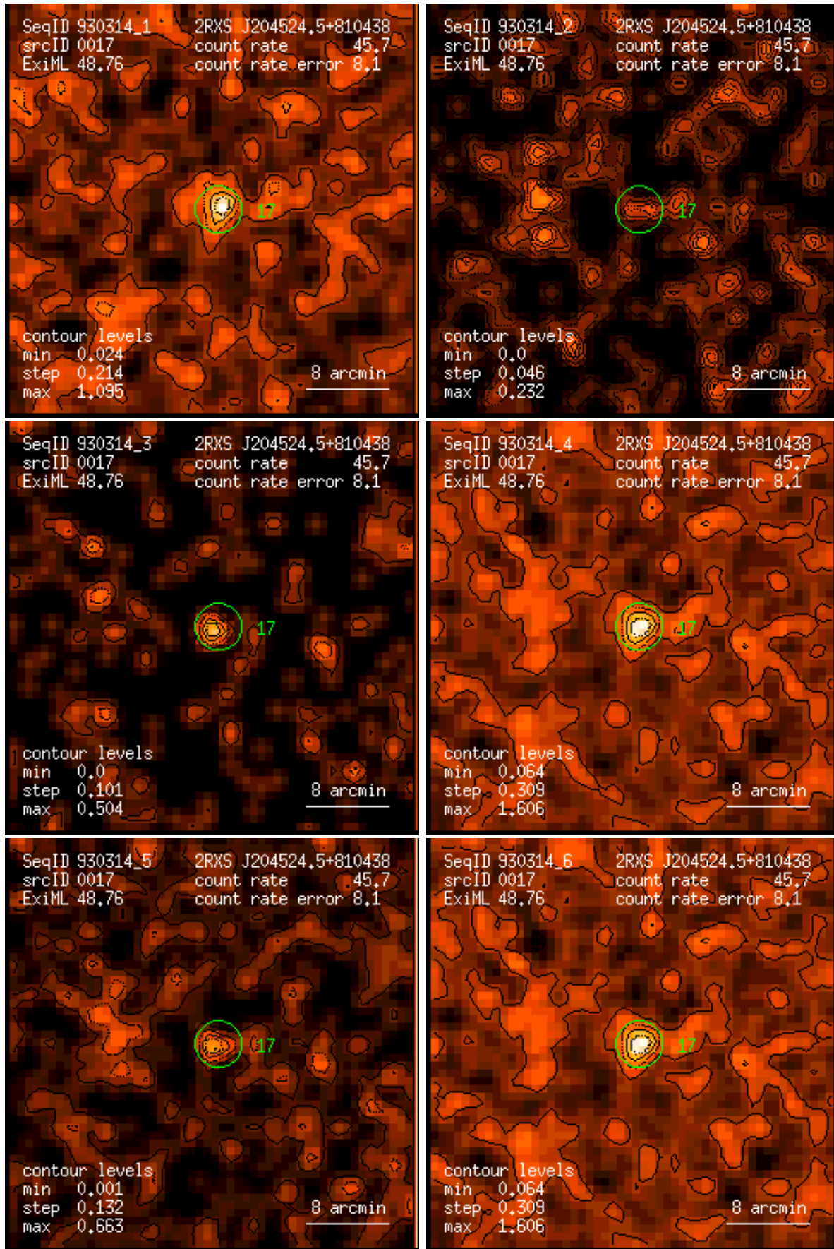
Figure 17: RASS 930314: detection 0017: band rate images, Gaussian filter: (1) PSPC channels 11 – 41, (2) 52 – 90, (3) 91 – 201, (4) 11 – 235, (5) 52 – 201, (6) 11 – 201. Broad band rates in counts/ks. Band rate contour levels in counts/ks/arcmin 2 .
