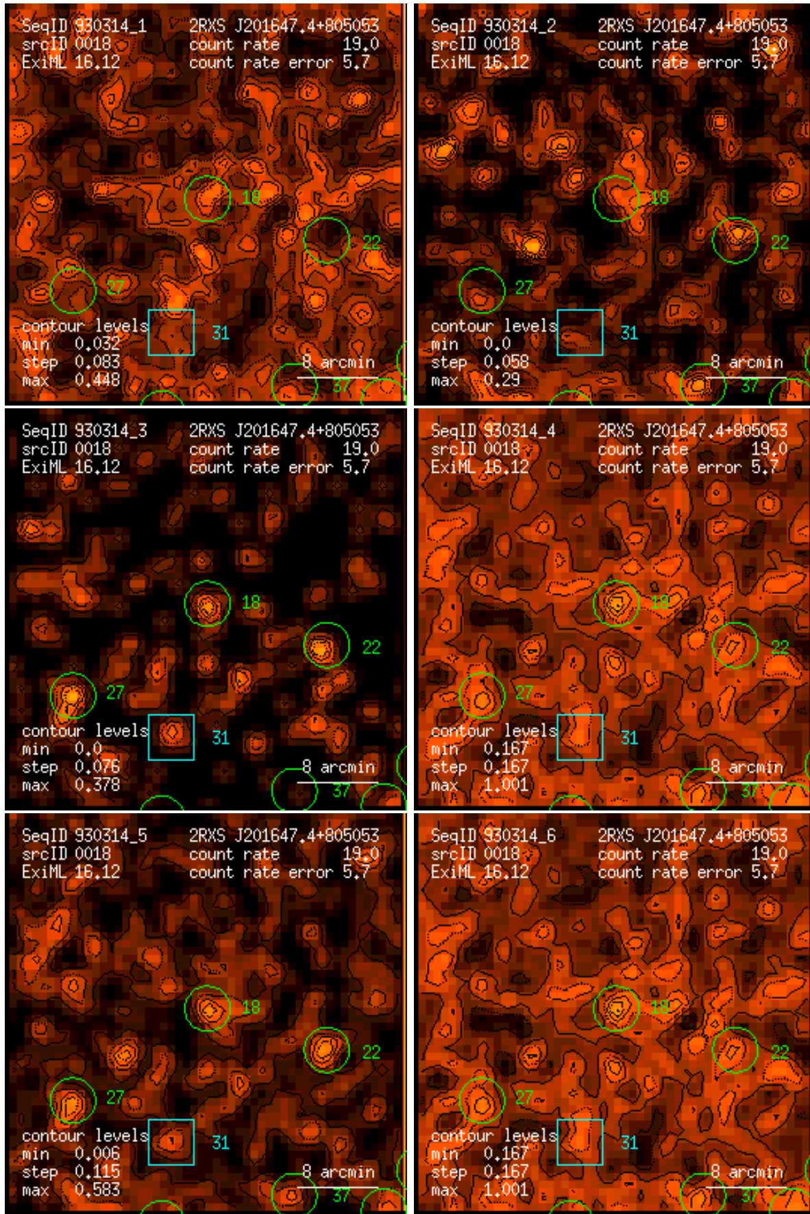
Figure 18: RASS 930314: detection 0018: band rate images, Gaussian filter: (1) PSPC channels 11 – 41, (2) 52 – 90, (3) 91 – 201, (4) 11 – 235, (5) 52 – 201, (6) 11 – 201. Broad band rates in counts/ks. Band rate contour levels in counts/ks/arcmin 2 .
