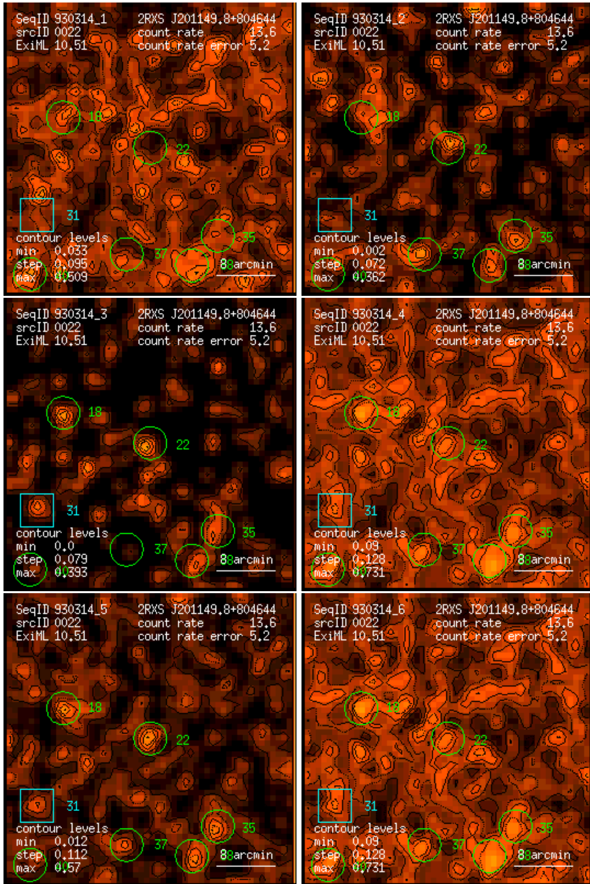
Figure 22: RASS 930314: detection 0022: band rate images, Gaussian filter: (1) PSPC channels 11 – 41, (2) 52 – 90, (3) 91 – 201, (4) 11 – 235, (5) 52 – 201, (6) 11 – 201. Broad band rates in counts/ks. Band rate contour levels in counts/ks/arcmin 2 .
