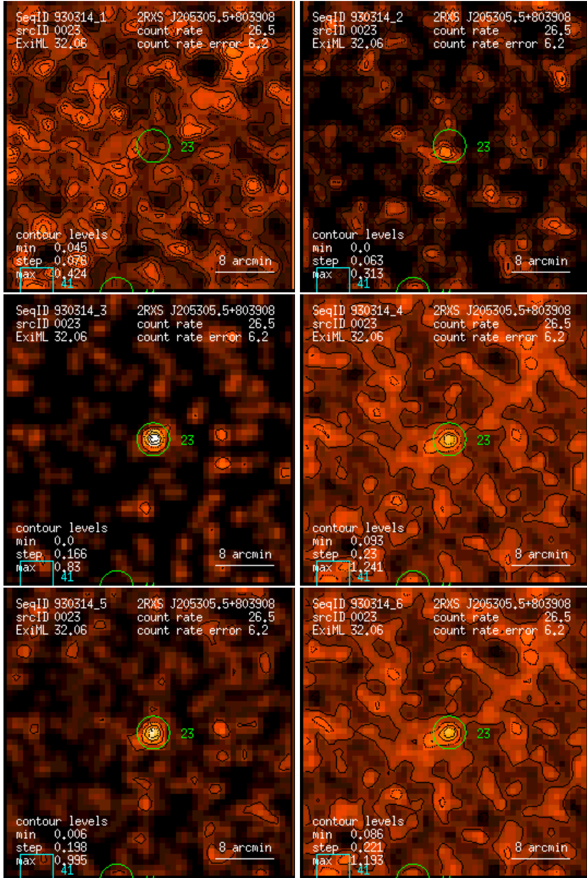
Figure 23: RASS 930314: detection 0023: band rate images, Gaussian filter: (1) PSPC channels 11 – 41, (2) 52 – 90, (3) 91 – 201, (4) 11 – 235, (5) 52 – 201, (6) 11 – 201. Broad band rates in counts/ks. Band rate contour levels in counts/ks/arcmin 2 .
