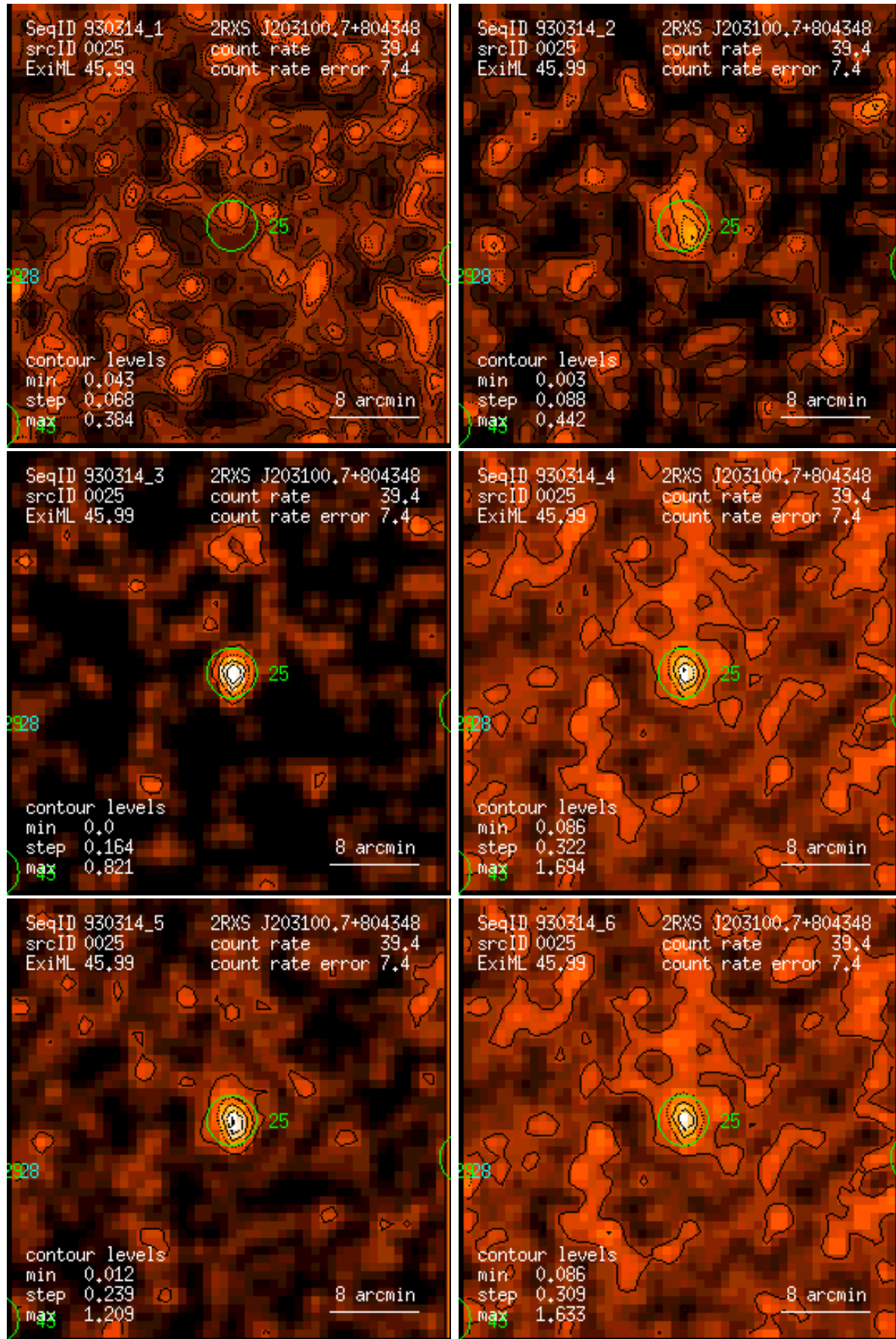
Figure 25: RASS 930314: detection 0025: band rate images, Gaussian filter: (1) PSPC channels 11 – 41, (2) 52 – 90, (3) 91 – 201, (4) 11 – 235, (5) 52 – 201, (6) 11 – 201. Broad band rates in counts/ks. Band rate contour levels in counts/ks/arcmin 2 .
