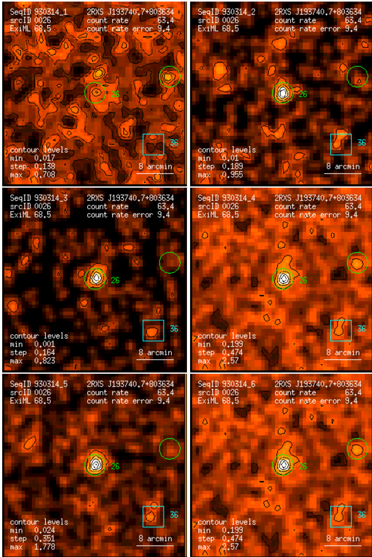
Figure 26: RASS 930314: detection 0026: band rate images, Gaussian filter: (1) PSPC channels 11 – 41, (2) 52 – 90, (3) 91 – 201, (4) 11 – 235, (5) 52 – 201, (6) 11 – 201. Broad band rates in counts/ks. Band rate contour levels in counts/ks/arcmin 2 .
