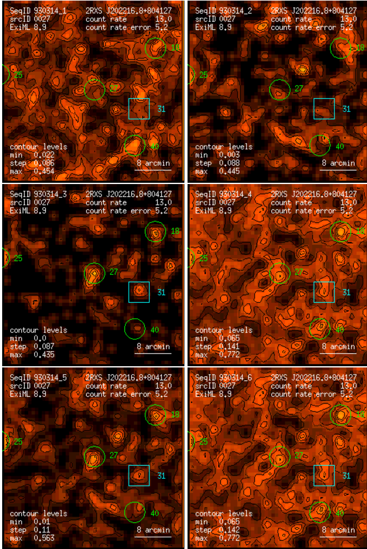
Figure 27: RASS 930314: detection 0027: band rate images, Gaussian filter: (1) PSPC channels 11 – 41, (2) 52 – 90, (3) 91 – 201, (4) 11 – 235, (5) 52 – 201, (6) 11 – 201. Broad band rates in counts/ks. Band rate contour levels in counts/ks/arcmin 2 .
