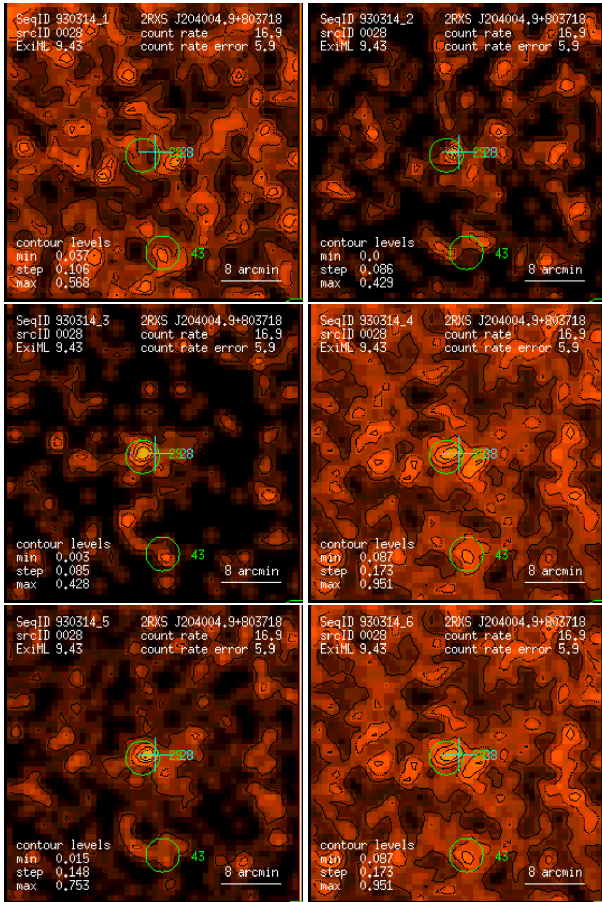
Figure 28: RASS 930314: detection 0028: band rate images, Gaussian filter: (1) PSPC channels 11 – 41, (2) 52 – 90, (3) 91 – 201, (4) 11 – 235, (5) 52 – 201, (6) 11 – 201. Broad band rates in counts/ks. Band rate contour levels in counts/ks/arcmin 2 .
