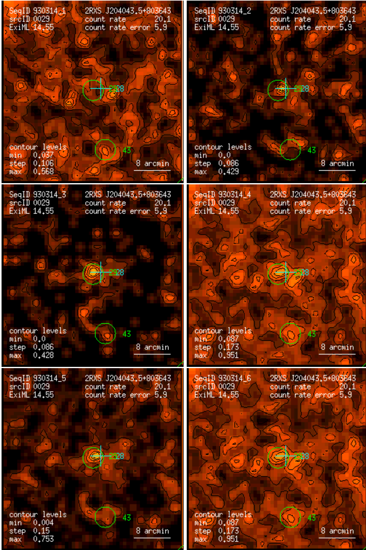
Figure 29: RASS 930314: detection 0029: band rate images, Gaussian filter: (1) PSPC channels 11 – 41, (2) 52 – 90, (3) 91 – 201, (4) 11 – 235, (5) 52 – 201, (6) 11 – 201. Broad band rates in counts/ks. Band rate contour levels in counts/ks/arcmin 2 .
