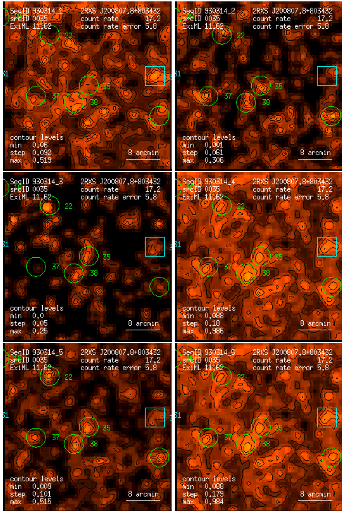
Figure 35: RASS 930314: detection 0035: band rate images, Gaussian filter: (1) PSPC channels 11 – 41, (2) 52 – 90, (3) 91 – 201, (4) 11 – 235, (5) 52 – 201, (6) 11 – 201. Broad band rates in counts/ks. Band rate contour levels in counts/ks/arcmin 2 .
