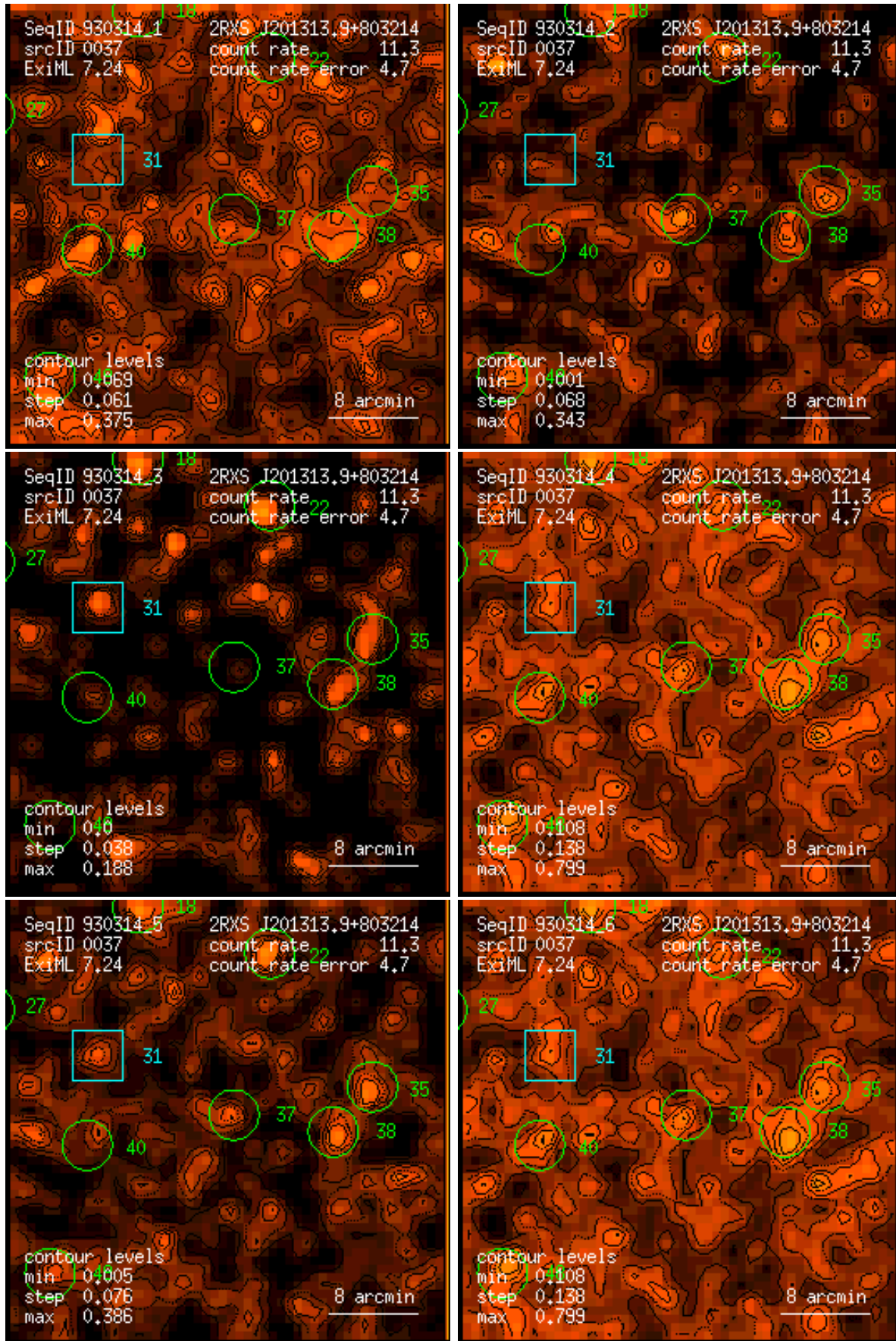
Figure 37: RASS 930314: detection 0037: band rate images, Gaussian filter: (1) PSPC channels 11 – 41, (2) 52 – 90, (3) 91 – 201, (4) 11 – 235, (5) 52 – 201, (6) 11 – 201. Broad band rates in counts/ks. Band rate contour levels in counts/ks/arcmin 2 .
