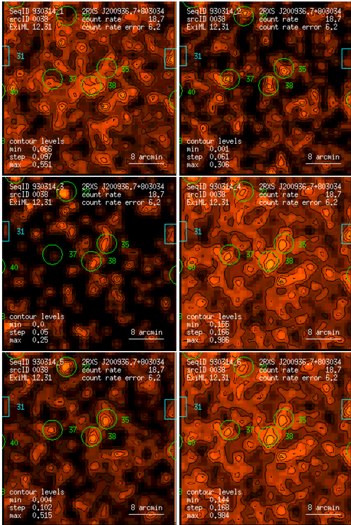
Figure 38: RASS 930314: detection 0038: band rate images, Gaussian filter: (1) PSPC channels 11 – 41, (2) 52 – 90, (3) 91 – 201, (4) 11 – 235, (5) 52 – 201, (6) 11 – 201. Broad band rates in counts/ks. Band rate contour levels in counts/ks/arcmin 2 .
