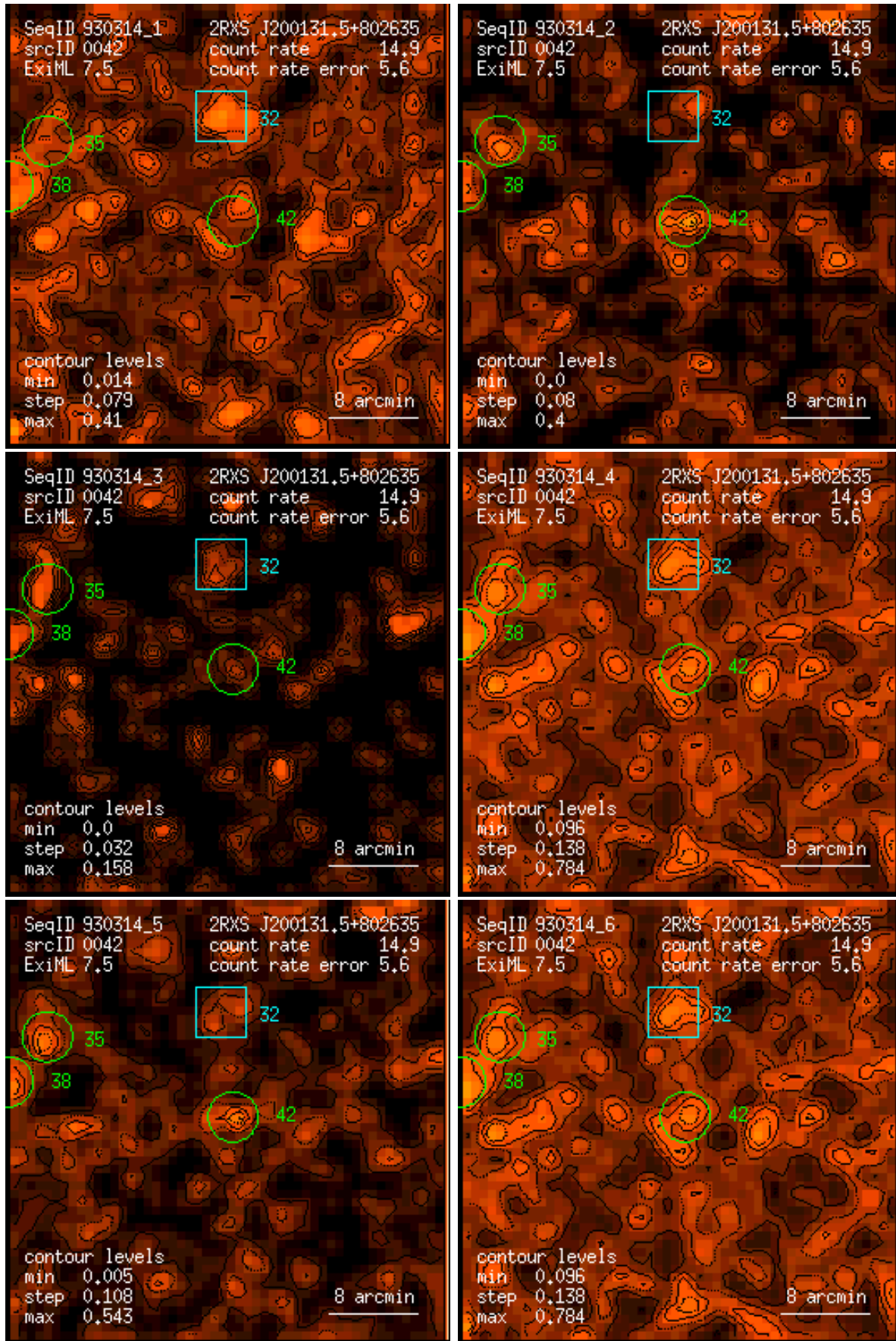
Figure 42: RASS 930314: detection 0042: band rate images, Gaussian filter: (1) PSPC channels 11 – 41, (2) 52 – 90, (3) 91 – 201, (4) 11 – 235, (5) 52 – 201, (6) 11 – 201. Broad band rates in counts/ks. Band rate contour levels in counts/ks/arcmin 2 .
