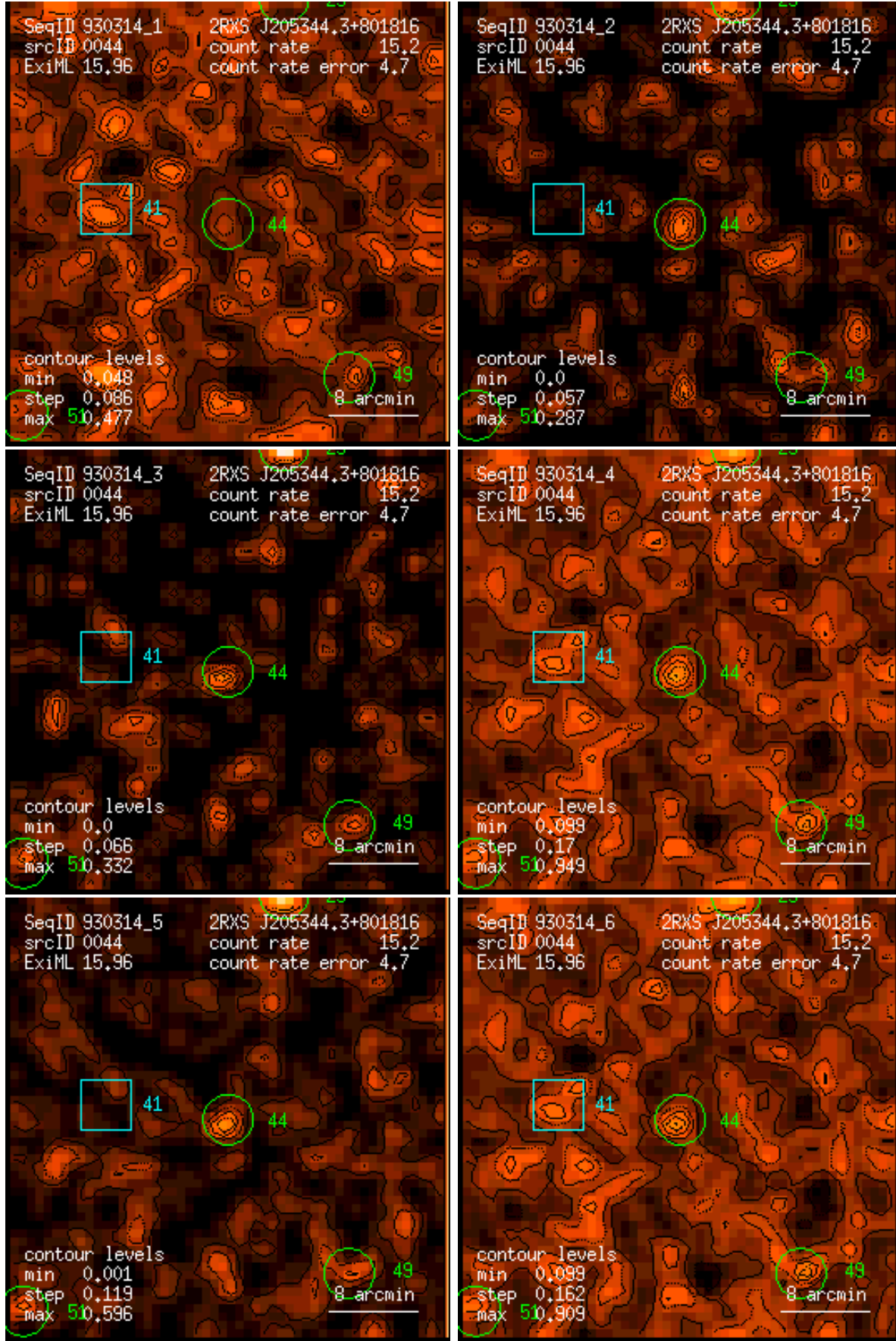
Figure 44: RASS 930314: detection 0044: band rate images, Gaussian filter: (1) PSPC channels 11 – 41, (2) 52 – 90, (3) 91 – 201, (4) 11 – 235, (5) 52 – 201, (6) 11 – 201. Broad band rates in counts/ks. Band rate contour levels in counts/ks/arcmin 2 .
