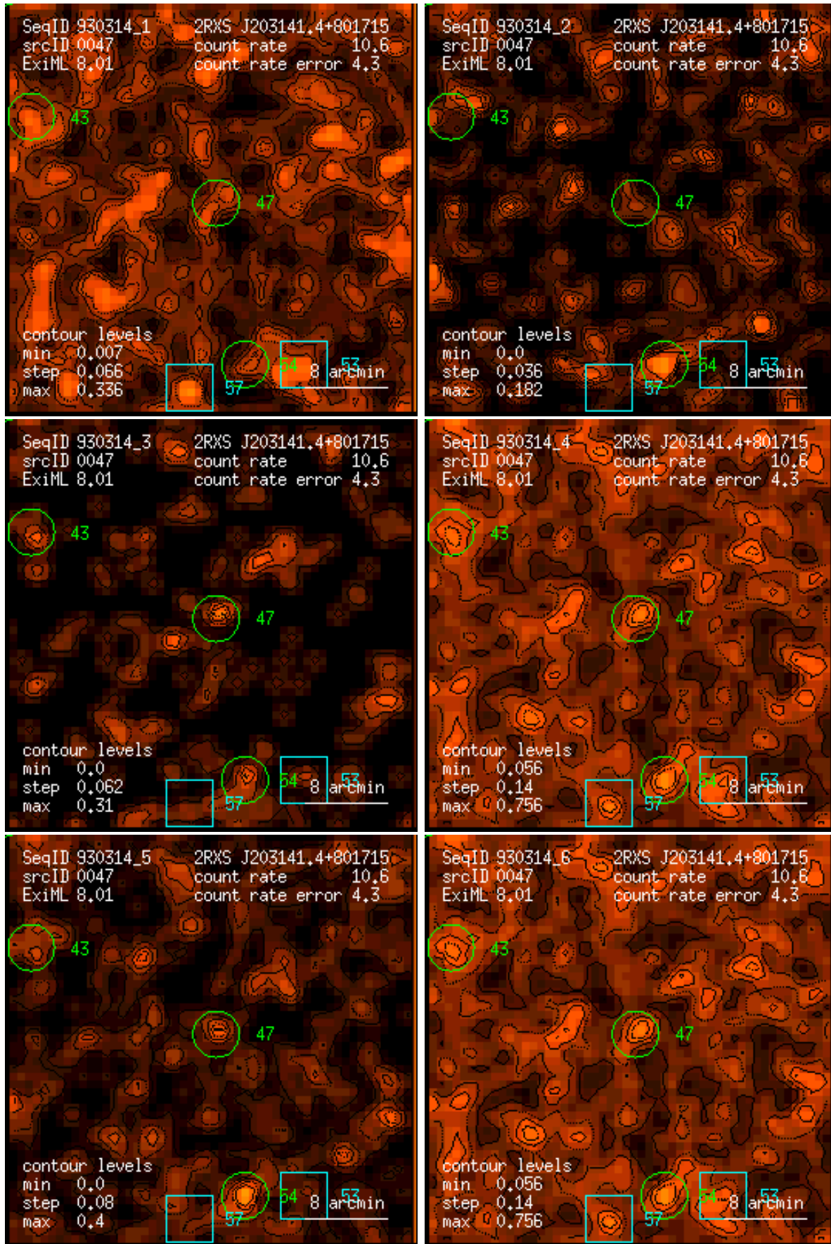
Figure 47: RASS 930314: detection 0047: band rate images, Gaussian filter: (1) PSPC channels 11 – 41, (2) 52 – 90, (3) 91 – 201, (4) 11 – 235, (5) 52 – 201, (6) 11 – 201. Broad band rates in counts/ks. Band rate contour levels in counts/ks/arcmin 2 .
