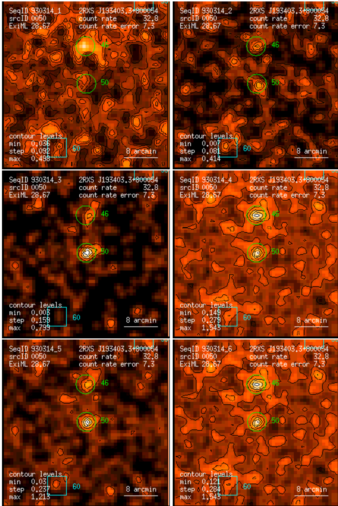
Figure 50: RASS 930314: detection 0050: band rate images, Gaussian filter: (1) PSPC channels 11 – 41, (2) 52 – 90, (3) 91 – 201, (4) 11 – 235, (5) 52 – 201, (6) 11 – 201. Broad band rates in counts/ks. Band rate contour levels in counts/ks/arcmin 2 .
