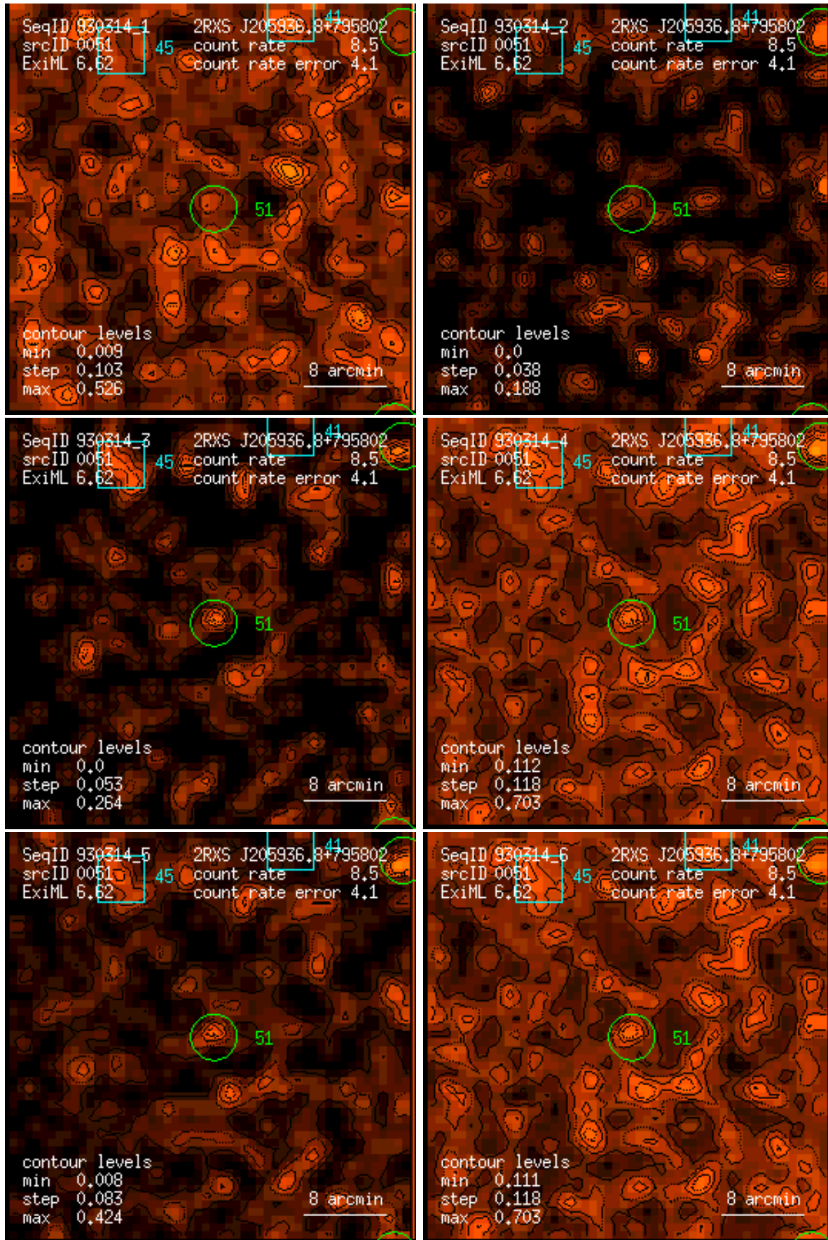
Figure 51: RASS 930314: detection 0051: band rate images, Gaussian filter: (1) PSPC channels 11 – 41, (2) 52 – 90, (3) 91 – 201, (4) 11 – 235, (5) 52 – 201, (6) 11 – 201. Broad band rates in counts/ks. Band rate contour levels in counts/ks/arcmin 2 .
