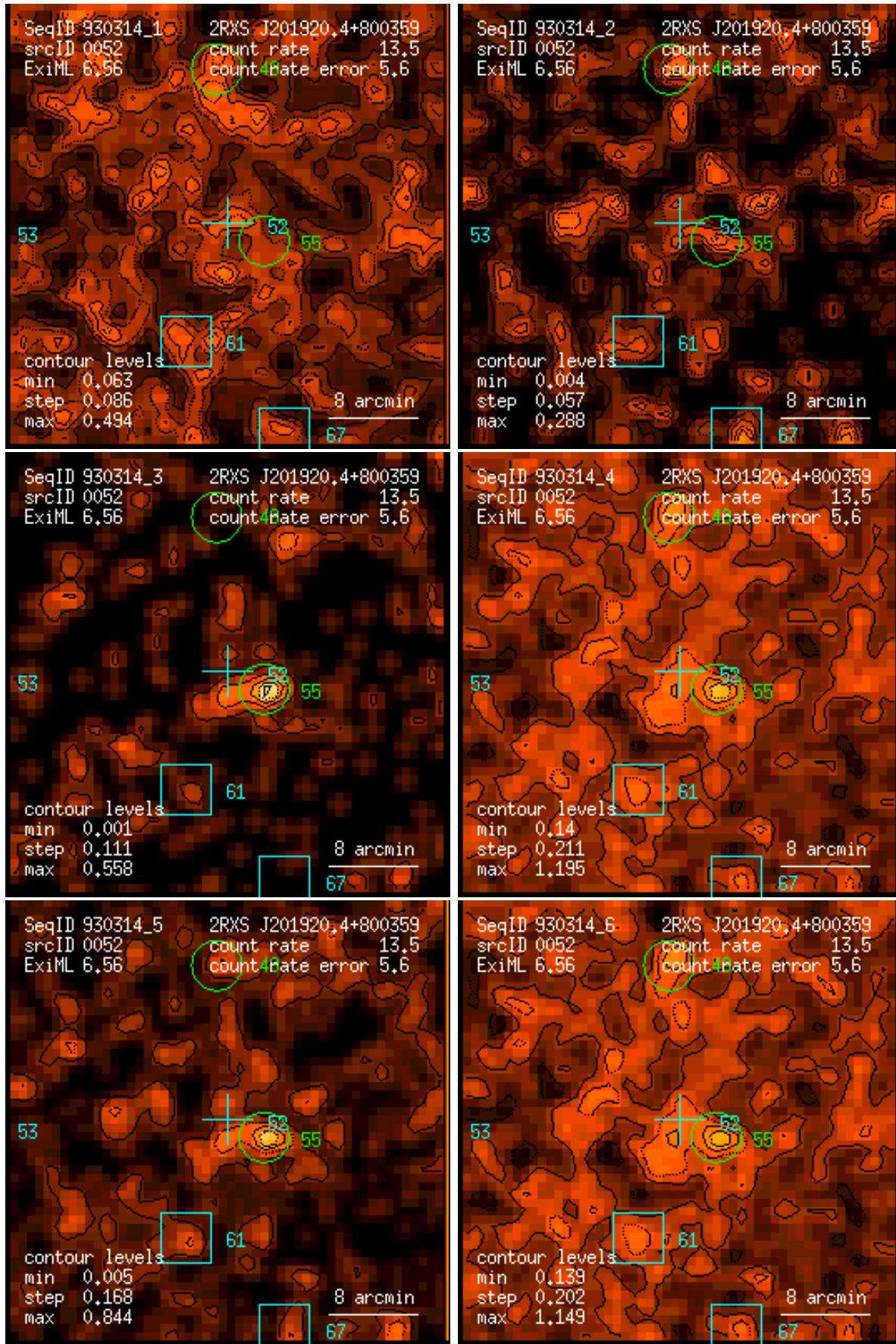
Figure 52: RASS 930314: detection 0052: band rate images, Gaussian filter: (1) PSPC channels 11 – 41, (2) 52 – 90, (3) 91 – 201, (4) 11 – 235, (5) 52 – 201, (6) 11 – 201. Broad band rates in counts/ks. Band rate contour levels in counts/ks/arcmin 2 .
