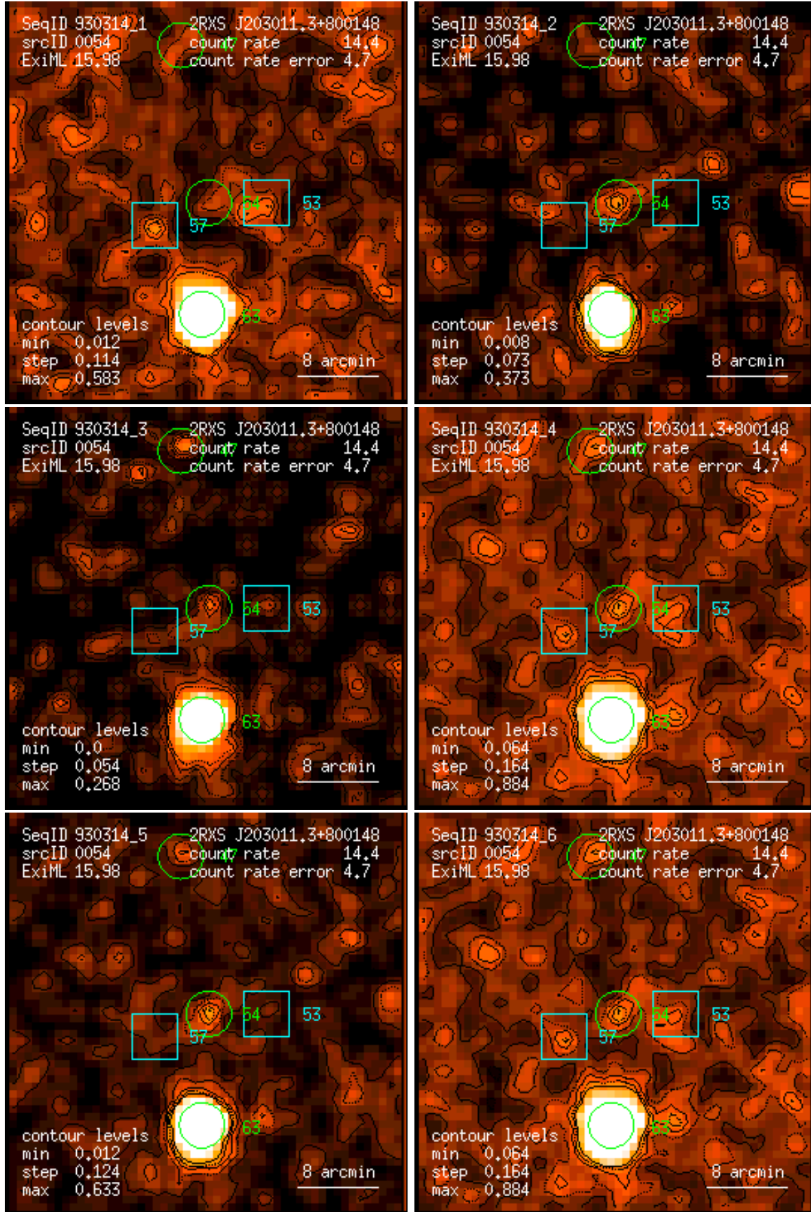
Figure 54: RASS 930314: detection 0054: band rate images, Gaussian filter: (1) PSPC channels 11 – 41, (2) 52 – 90, (3) 91 – 201, (4) 11 – 235, (5) 52 – 201, (6) 11 – 201. Broad band rates in counts/ks. Band rate contour levels in counts/ks/arcmin 2 .
