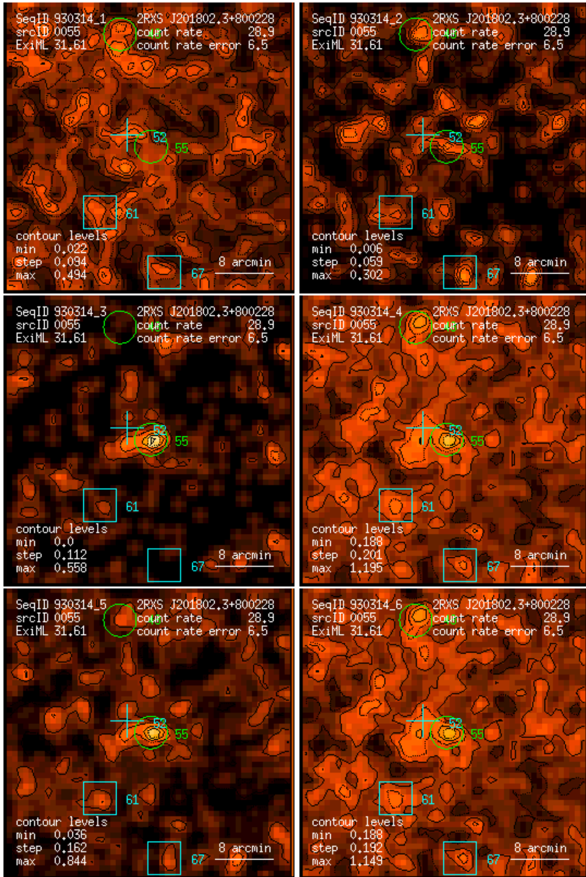
Figure 55: RASS 930314: detection 0055: band rate images, Gaussian filter: (1) PSPC channels 11 – 41, (2) 52 – 90, (3) 91 – 201, (4) 11 – 235, (5) 52 – 201, (6) 11 – 201. Broad band rates in counts/ks. Band rate contour levels in counts/ks/arcmin 2 .
