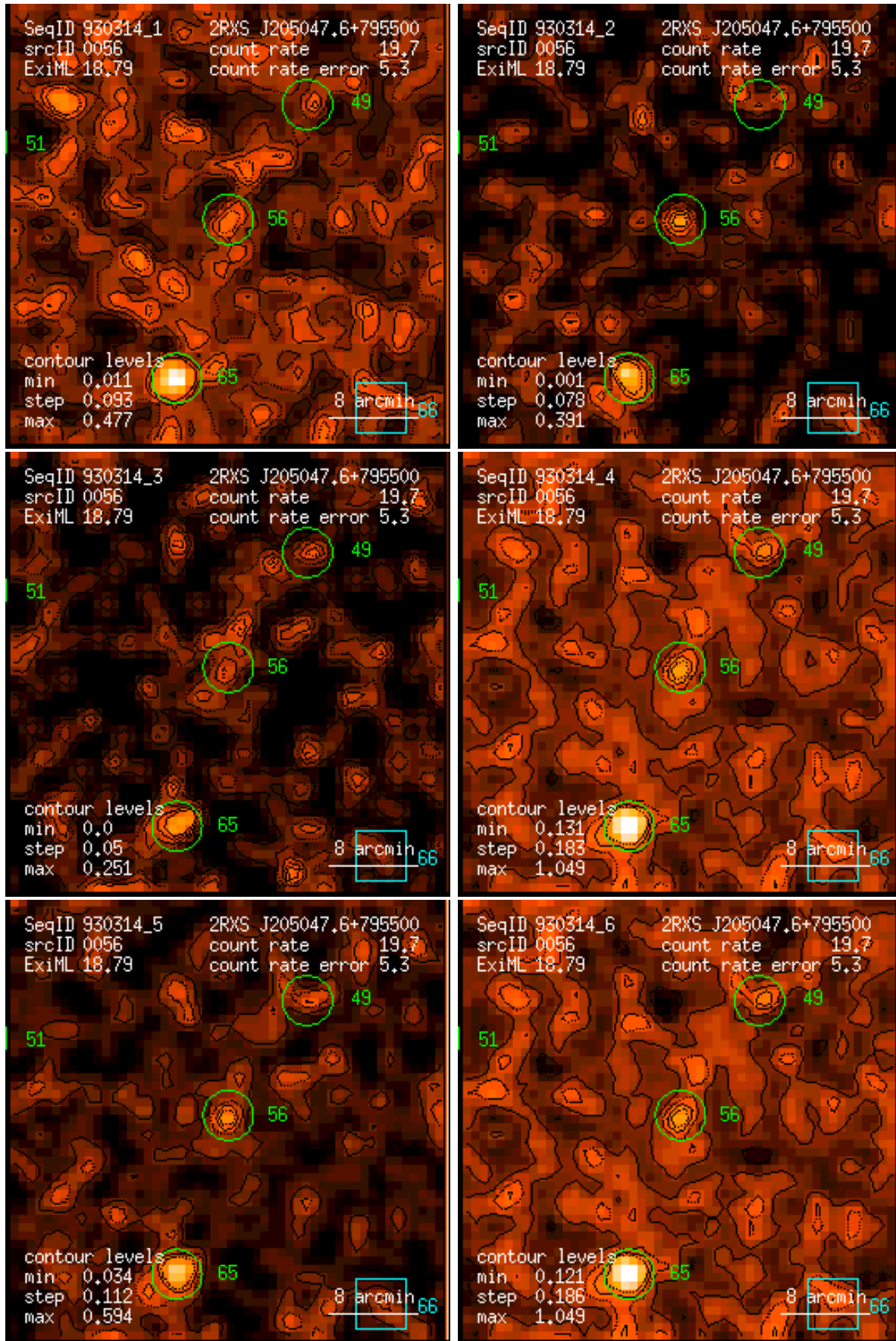
Figure 56: RASS 930314: detection 0056: band rate images, Gaussian filter: (1) PSPC channels 11 – 41, (2) 52 – 90, (3) 91 – 201, (4) 11 – 235, (5) 52 – 201, (6) 11 – 201. Broad band rates in counts/ks. Band rate contour levels in counts/ks/arcmin 2 .
