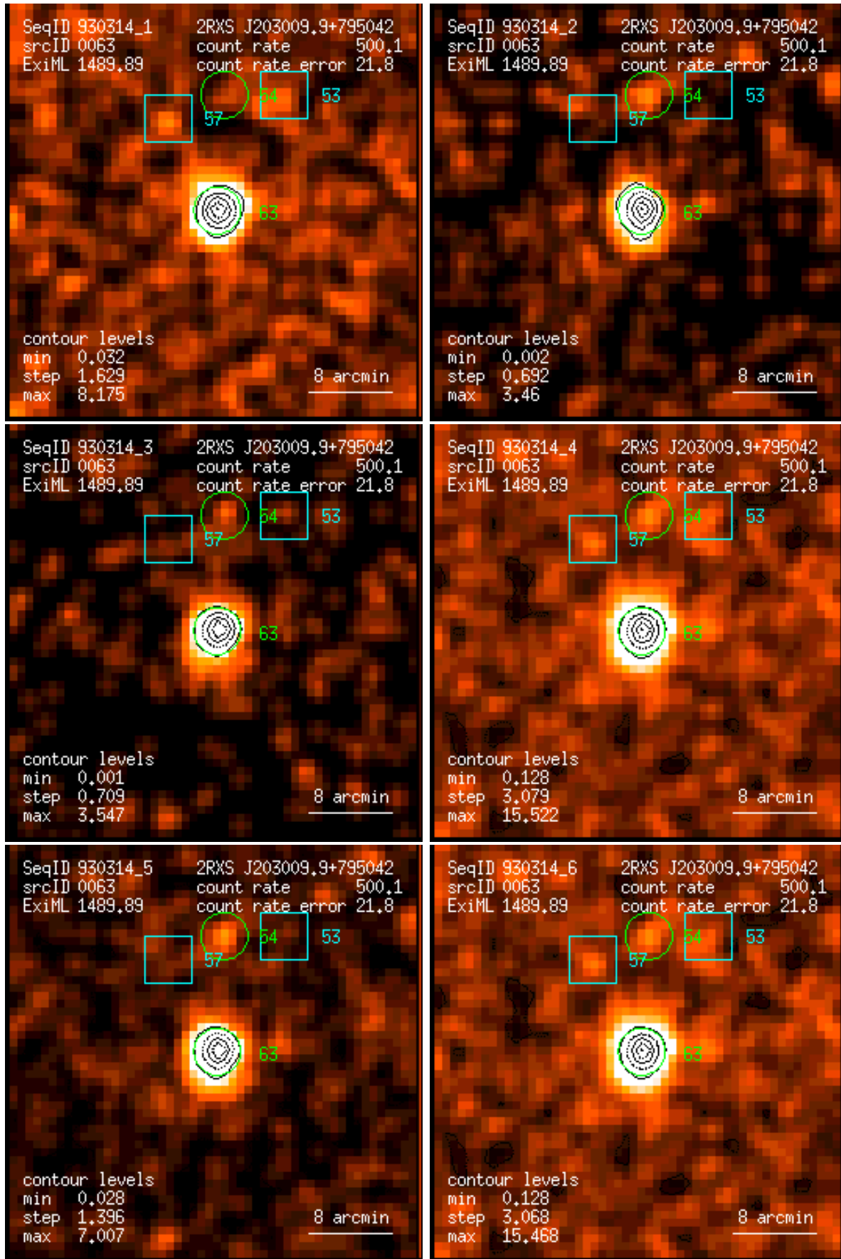
Figure 63: RASS 930314: detection 0063: band rate images, Gaussian filter: (1) PSPC channels 11 – 41, (2) 52 – 90, (3) 91 – 201, (4) 11 – 235, (5) 52 – 201, (6) 11 – 201. Broad band rates in counts/ks. Band rate contour levels in counts/ks/arcmin 2 .
