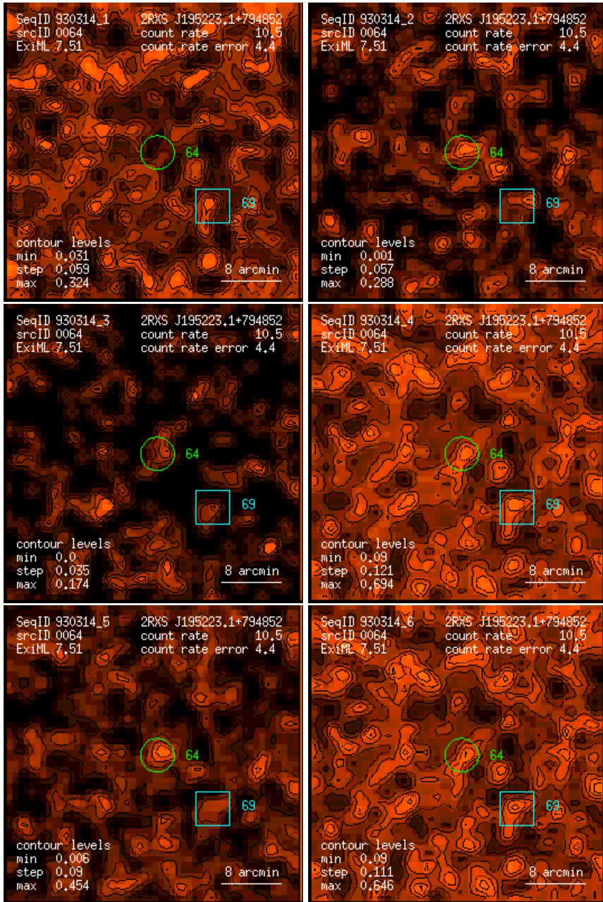
Figure 64: RASS 930314: detection 0064: band rate images, Gaussian filter: (1) PSPC channels 11 – 41, (2) 52 – 90, (3) 91 – 201, (4) 11 – 235, (5) 52 – 201, (6) 11 – 201. Broad band rates in counts/ks. Band rate contour levels in counts/ks/arcmin 2 .
