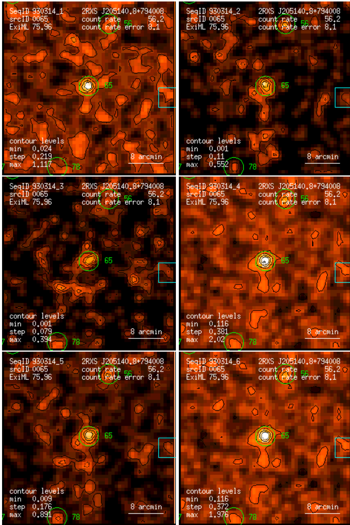
Figure 65: RASS 930314: detection 0065: band rate images, Gaussian filter: (1) PSPC channels 11 – 41, (2) 52 – 90, (3) 91 – 201, (4) 11 – 235, (5) 52 – 201, (6) 11 – 201. Broad band rates in counts/ks. Band rate contour levels in counts/ks/arcmin 2 .
