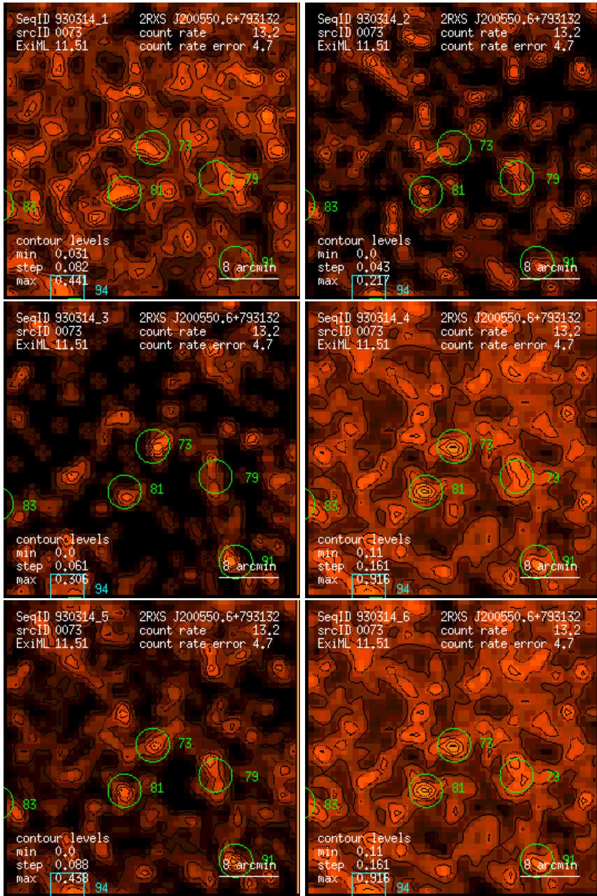
Figure 73: RASS 930314: detection 0073: band rate images, Gaussian filter: (1) PSPC channels 11 – 41, (2) 52 – 90, (3) 91 – 201, (4) 11 – 235, (5) 52 – 201, (6) 11 – 201. Broad band rates in counts/ks. Band rate contour levels in counts/ks/arcmin 2 .
