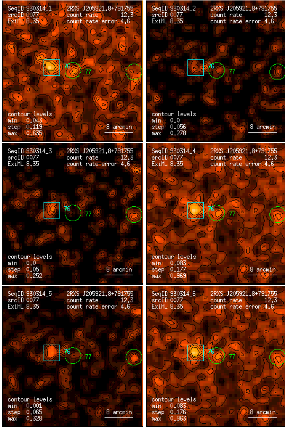
Figure 77: RASS 930314: detection 0077: band rate images, Gaussian filter: (1) PSPC channels 11 – 41, (2) 52 – 90, (3) 91 – 201, (4) 11 – 235, (5) 52 – 201, (6) 11 – 201. Broad band rates in counts/ks. Band rate contour levels in counts/ks/arcmin 2 .
