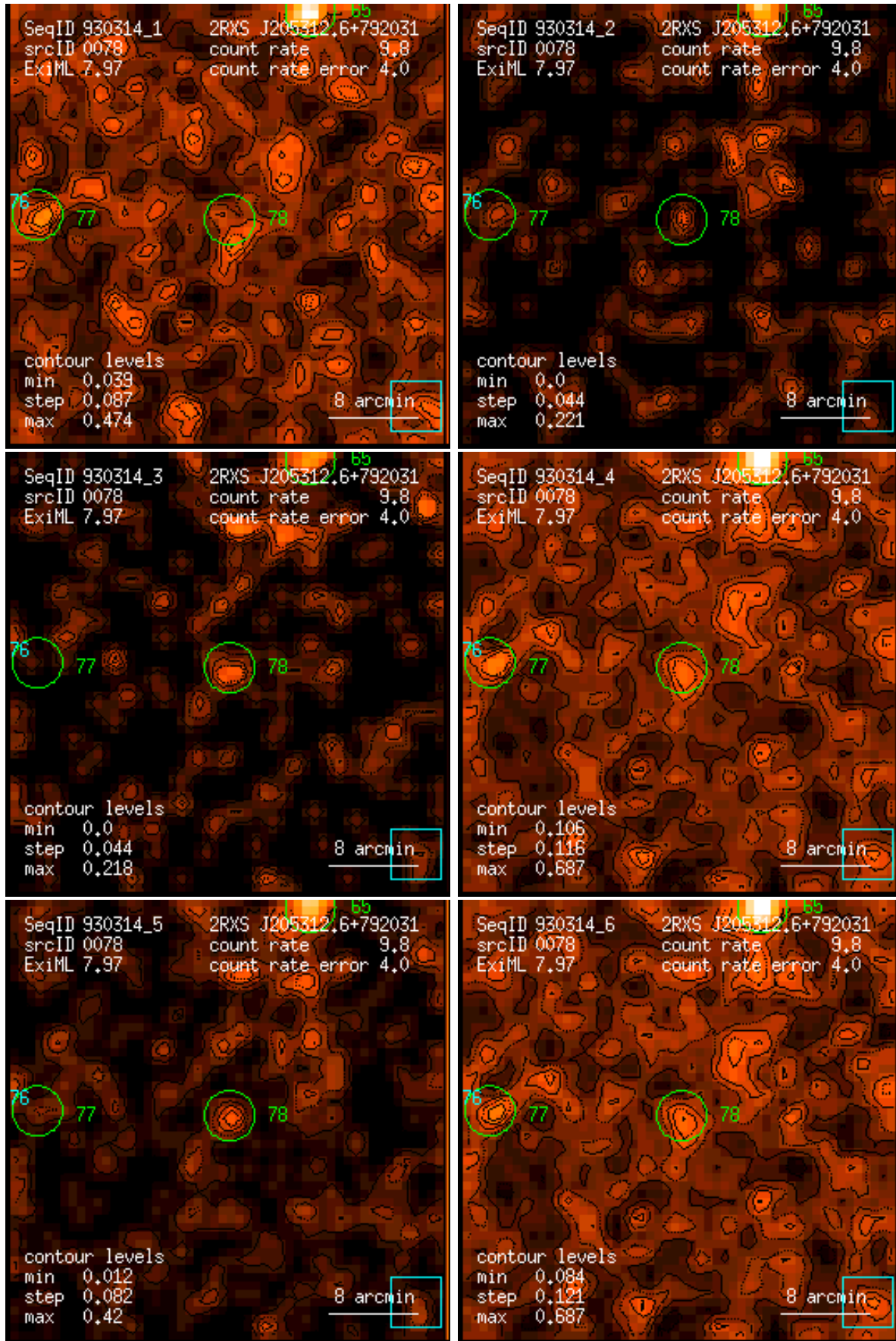
Figure 78: RASS 930314: detection 0078: band rate images, Gaussian filter: (1) PSPC channels 11 – 41, (2) 52 – 90, (3) 91 – 201, (4) 11 – 235, (5) 52 – 201, (6) 11 – 201. Broad band rates in counts/ks. Band rate contour levels in counts/ks/arcmin 2 .
