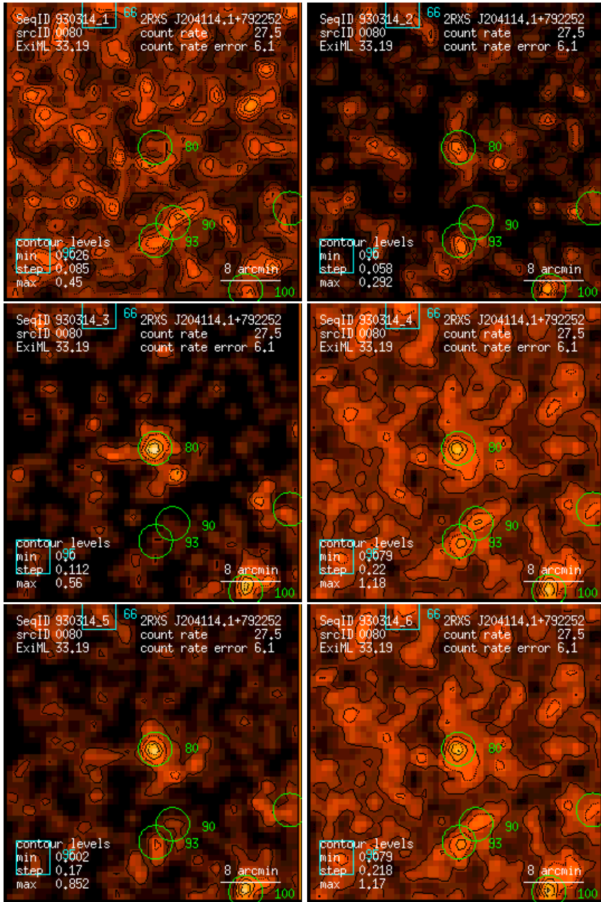
Figure 80: RASS 930314: detection 0080: band rate images, Gaussian filter: (1) PSPC channels 11 – 41, (2) 52 – 90, (3) 91 – 201, (4) 11 – 235, (5) 52 – 201, (6) 11 – 201. Broad band rates in counts/ks. Band rate contour levels in counts/ks/arcmin 2 .
