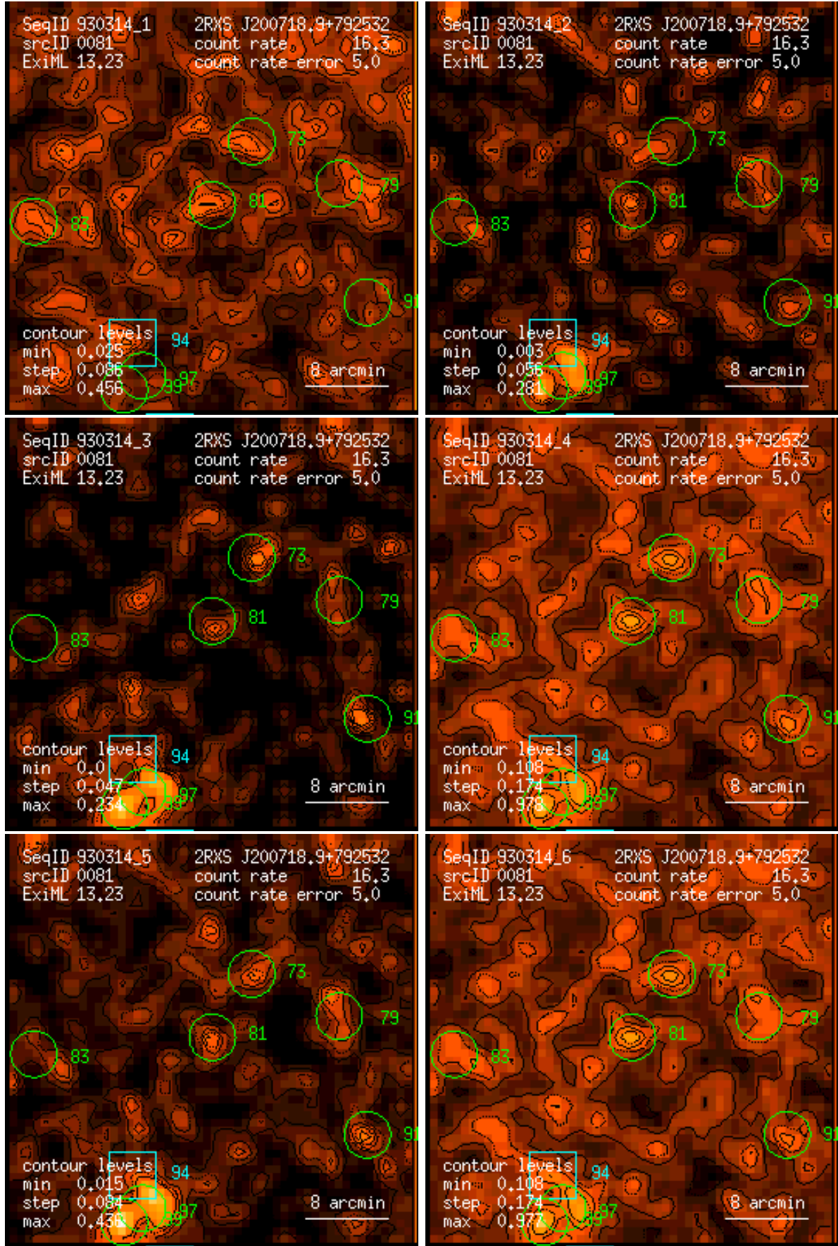
Figure 81: RASS 930314: detection 0081: band rate images, Gaussian filter: (1) PSPC channels 11 – 41, (2) 52 – 90, (3) 91 – 201, (4) 11 – 235, (5) 52 – 201, (6) 11 – 201. Broad band rates in counts/ks. Band rate contour levels in counts/ks/arcmin 2 .
