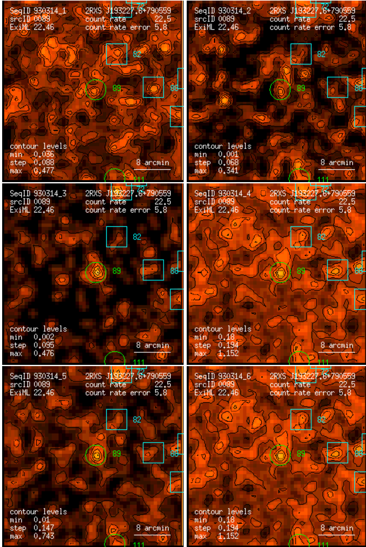
Figure 89: RASS 930314: detection 0089: band rate images, Gaussian filter: (1) PSPC channels 11 – 41, (2) 52 – 90, (3) 91 – 201, (4) 11 – 235, (5) 52 – 201, (6) 11 – 201. Broad band rates in counts/ks. Band rate contour levels in counts/ks/arcmin 2 .
